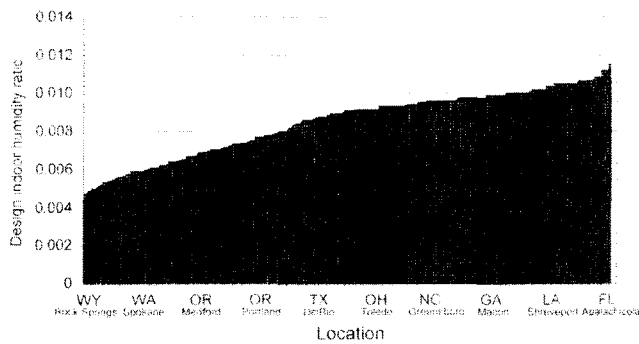
Figure 1 Design indoor humidity ratios as used in draft ASHRAE Standard 152P.
