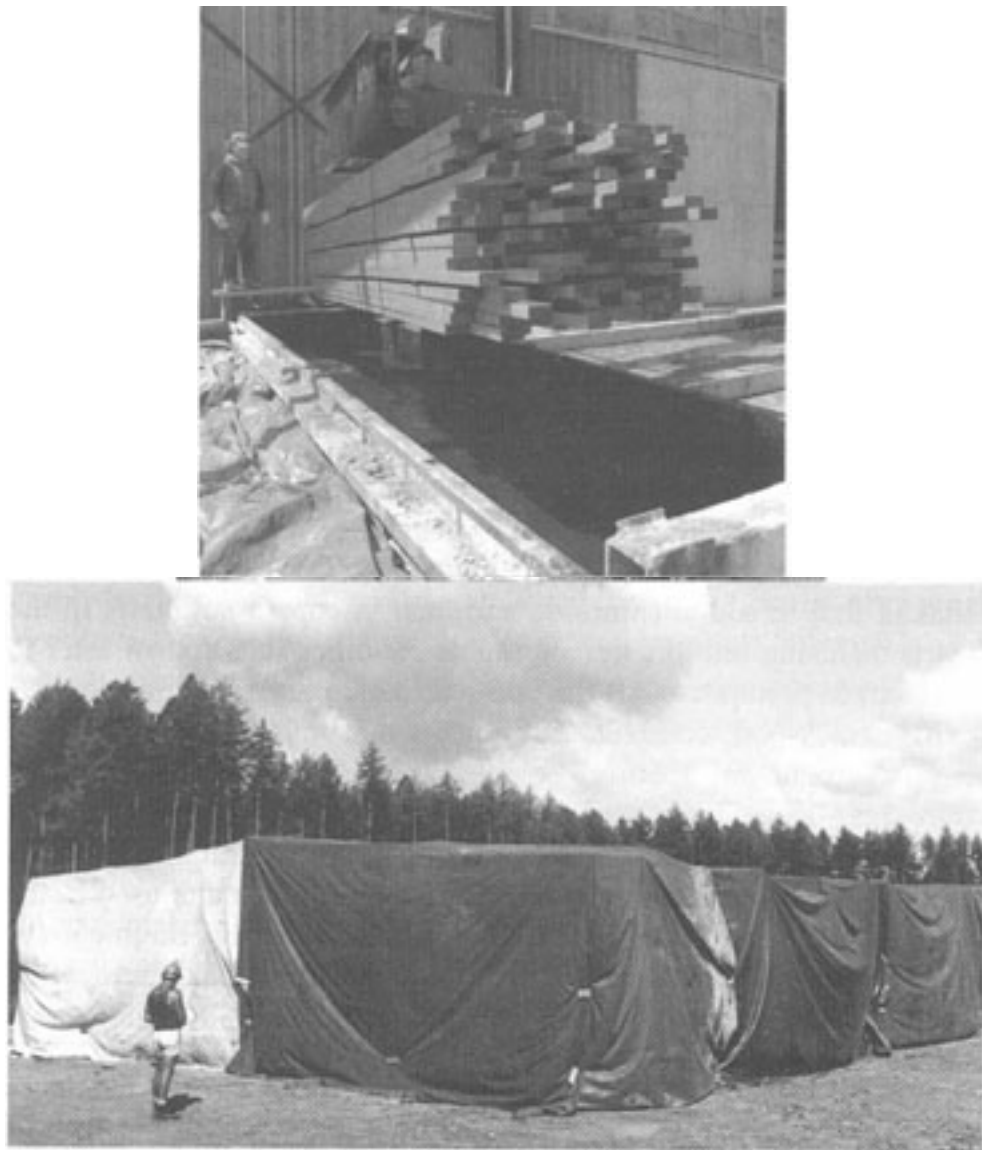
Figure 9.6. (a) Timber about to be immersed in a boron dip tank. Concrete drip storage area to the right. (b) Block stacked and covered timber is held for 4-8 weeks to allow salts to diffuse into the core.
