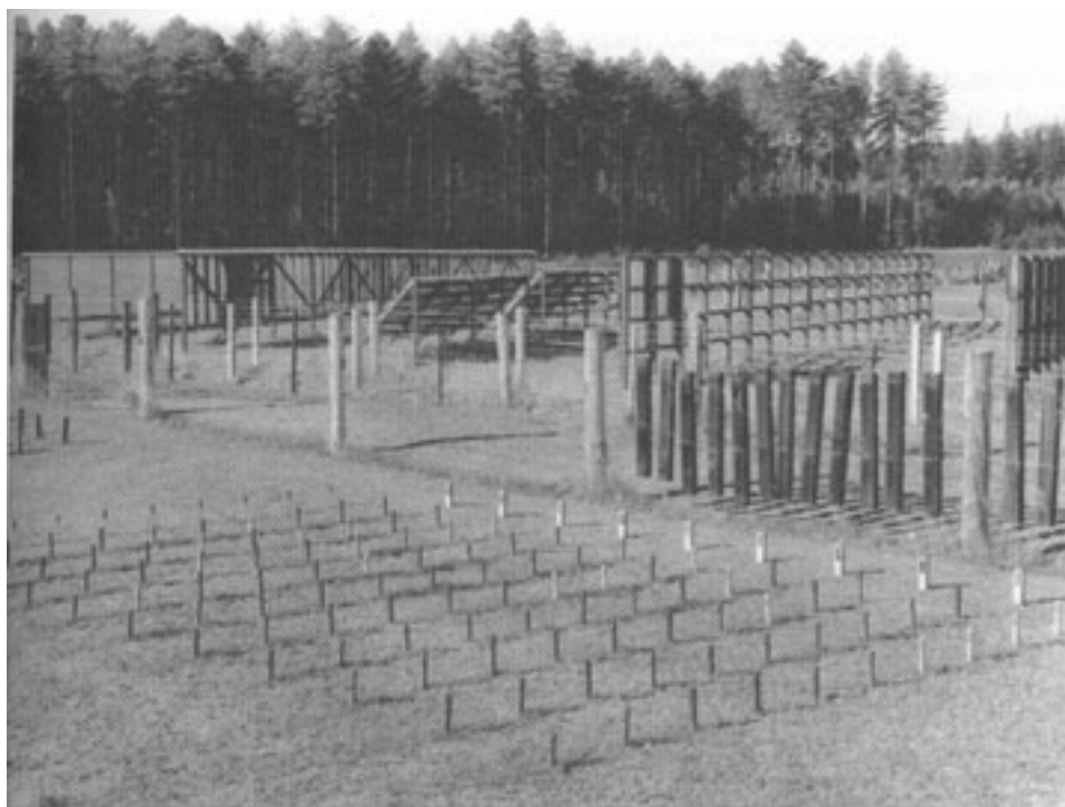
Figure 9. Field tests, also known as graveyard trials, as used to establish the durability of untreated heartwood of various timbers and also to determine the effectiveness of a variety of preservative systems (unpubl. courtesy New Zealand Forest Research Institute).
