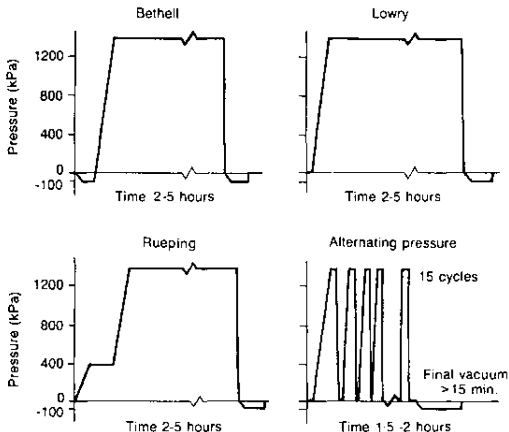
Figure 9.5. Time-pressure impregnation treatments
