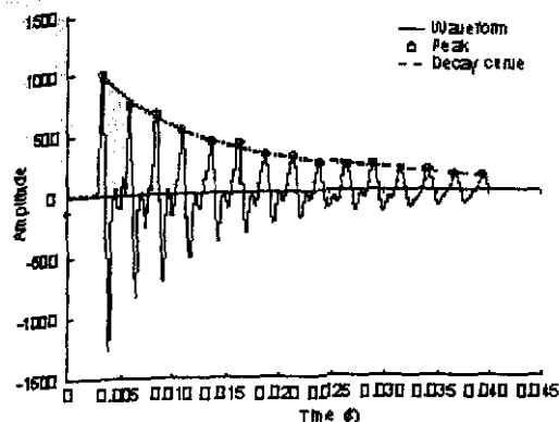
Figure 1. Typical waveform observed in acoustic testing of green ponderosa pine 2x4's.
