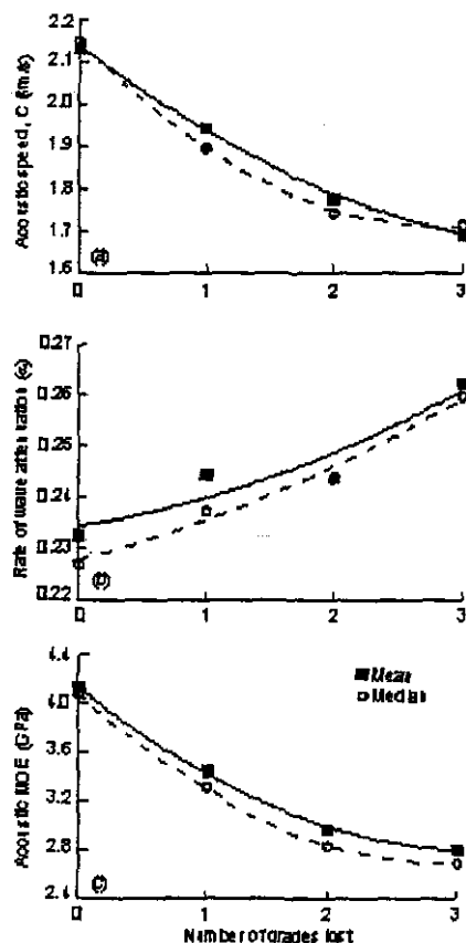
Figure 3. Relationship between (a) acoustic speed lengthwise, (b) rate of wave attenuation, and (c) acoustic modulus of elasticity (MOE) of green ponderosa pine 2 by 4's and the number of grades lost from warp during kiln drying.
