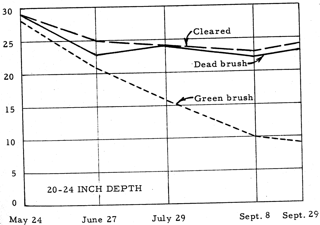
Figure 1. --Trend of soil moisture at depths of 10-14 and 20-24 inches.
