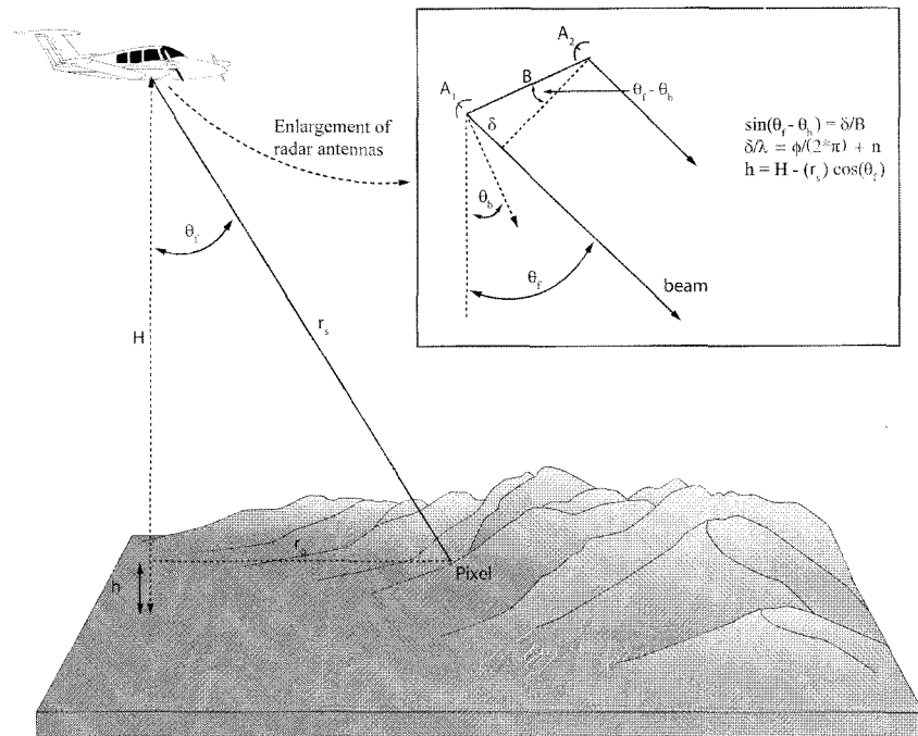
Figure 3-10. Geometry of RADAR interferometry. Adapted from Mercer (2004).
