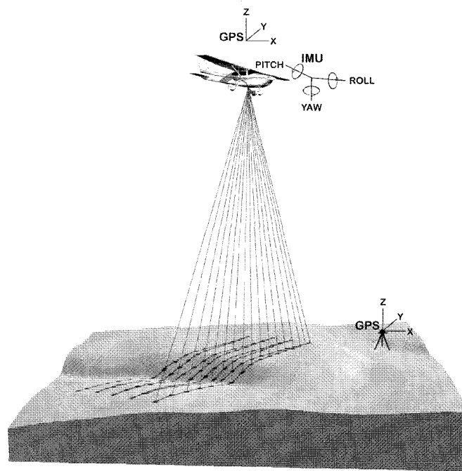
Figure 3-2. An illustration of airborne laser scanning.
