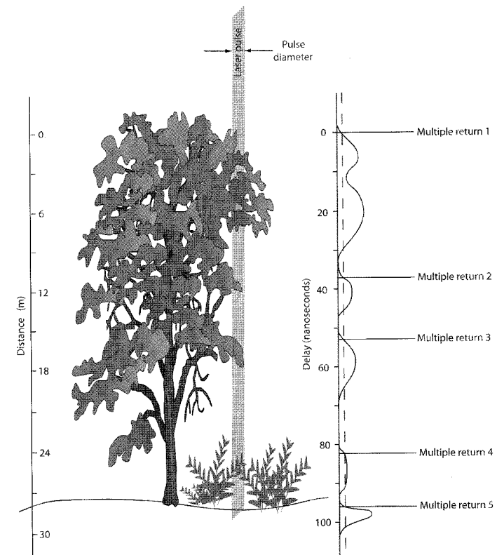
Figure 3-1. LIDAR remote sensing of vegetation. As the laser pulse passes through tree canopy, a signal is returned to the sensor. The leading edges of peaks in the returned signal correspond to multiple returns. Adapted from Lefsky et al. (2002).
