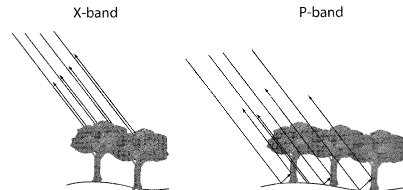
Figure 3-9. Short wavelength X-band RADAR energy reflects from canopy surface while long wavelength P-band energy penetrates through canopy and reflects from stems and terrain surface. Adapted from Moreira et al. (2001).
