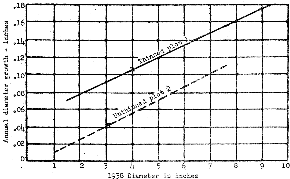
Figure 2.--Regression of annual diameter growth (1938-48) on diameter (1938): Ochoco thinning plots 1 and 2
