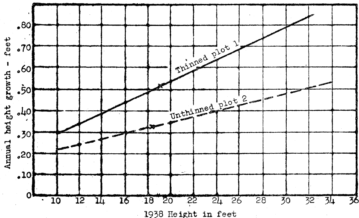
Figure 3.--Regression of annual height growth (1938-48) on height (1938): Ochoco thinning plots 1 and 2
