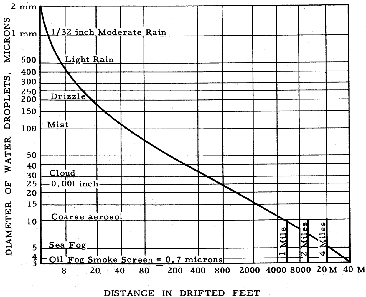
Figure 1.--Drift of various size water droplets while settling 10 feet in straight air flow of 3 miles per hour. From: Brooks, F. A., The drifting of poisonous dusts applied by air-planes and land rigs. Agricultural Engineering. 28(6): 234. June 1947. Reproduced by permission of Agricultural Engineering.
