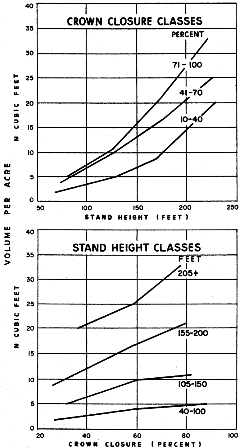
Figure 1. ---Relation of stand volume to stand height and crown closure (plotting of basic data).
