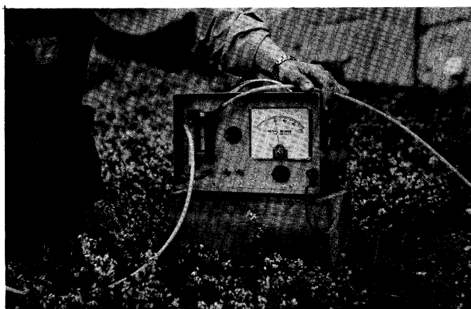
Figure 1. - Fumiscopes used to measure concentrations of methyl bromide.
