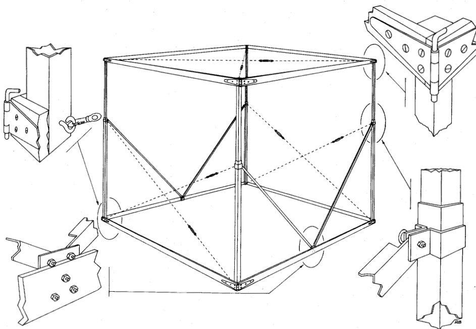
Figure 5. - Diagrammatic view of modified fumigation chamber showing construction details.
