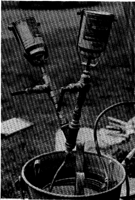
Figure 9. – Gas applicator and volatilizer used for dispensing ½-pound and 1-pound amounts of methyl bromide.
