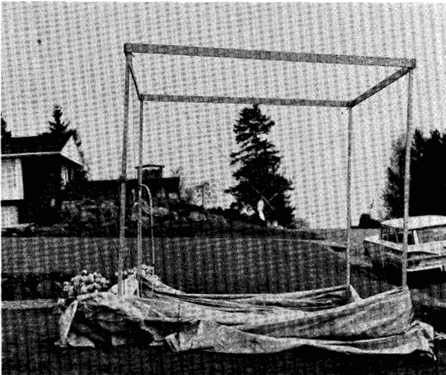
Figure 4. - The 10' x 10' x 10' cubical fumigation chamber; A, the uncovered frame; B, completed chamber.
