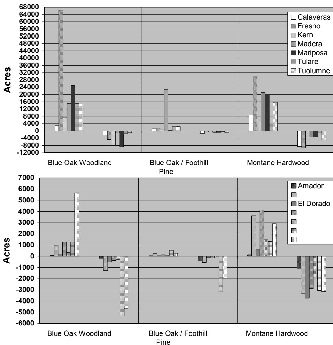
Figure 3 —Acres of classified change by hardwood type and county.
