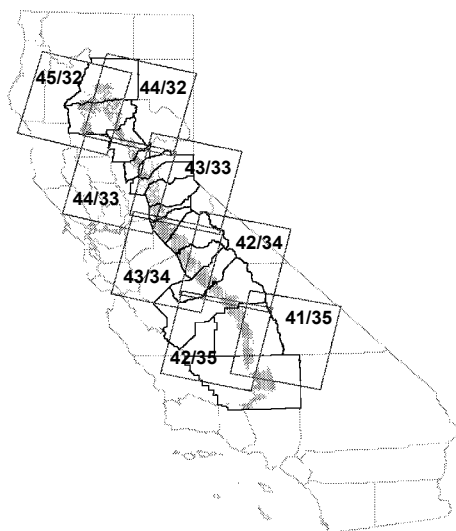
Figure 2 —Location of project area and TM scenes. Grey area is hardwood rangeland.
