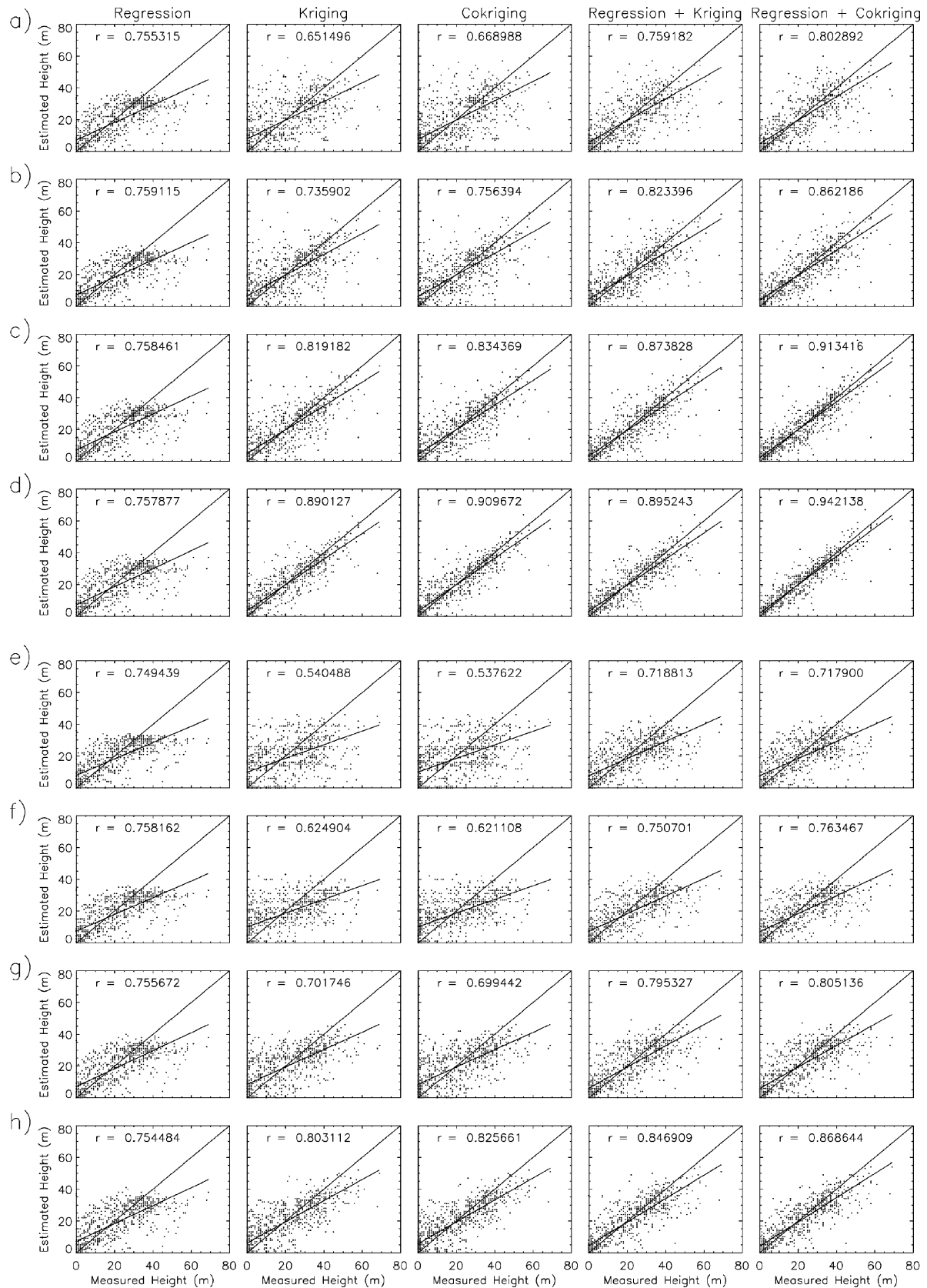
Fig. 6. Scatterplots of measured vs. estimated height values from the five models tested, for the eight sampling strategies tested: (a) 2000-m transect, (b) 1000-m transect, (c) 500-m transect, (d) 250-m transect, (e) 2000-m point, (f) 1000-m point, (g) 500-m point, and (h) 250-m point. Locations of the plotted values ( N=700 ) are shown in Fig. 3.
