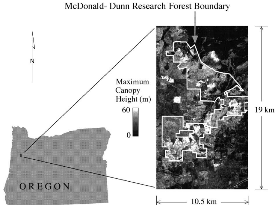
Fig. 1. Study area location and maximum canopy height image measured by lidar.
