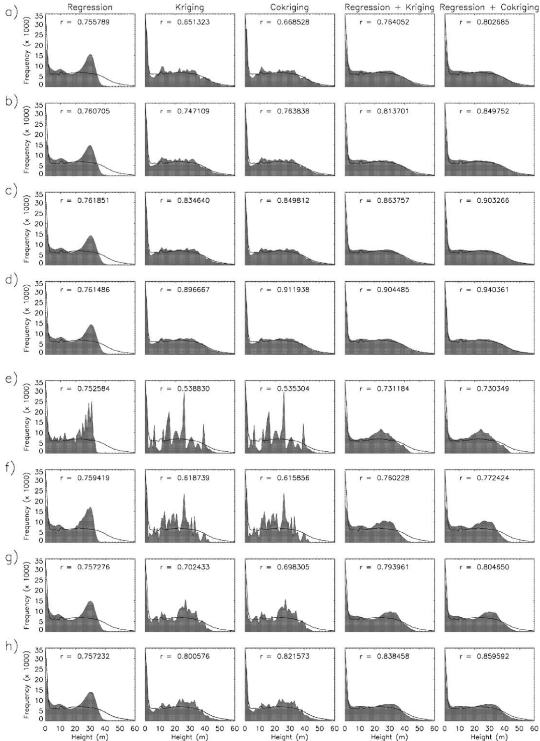
Fig. 5. Histograms of the entire population of estimated height values (shaded in gray, N=337,464 ) from the five models tested, for the eight sampling strategies tested: (a) 2000-m transect, (b) 1000-m transect, (c) 500-m transect, (d) 250-m transect, (e) 2000-m point, (f) 1000-m point, (g) 500-m point, and (h) 250-m point. The outline of the measured height value histogram is plotted over each estimated height value histogram for comparison.
