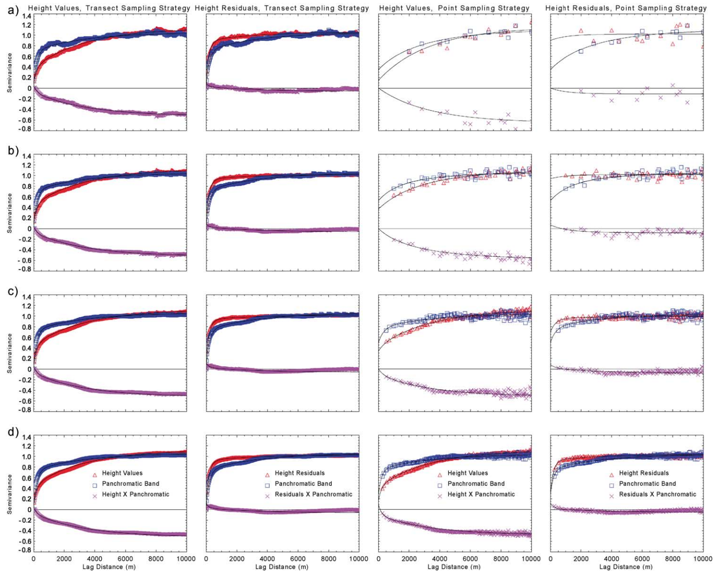
Fig. 4. Sample and model semivariograms of the primary and secondary datasets, from transect and point sampling intervals of: (a) 2000, (b) 1000, (c) 500, and (d) 250 m. The lines plotted over the sample semivariograms are the fitted model semivariograms. The cross-semivariograms are negative because the primary variables (height or height residuals) are negatively correlated to the secondary variable (ETM+ panchromatic band).
