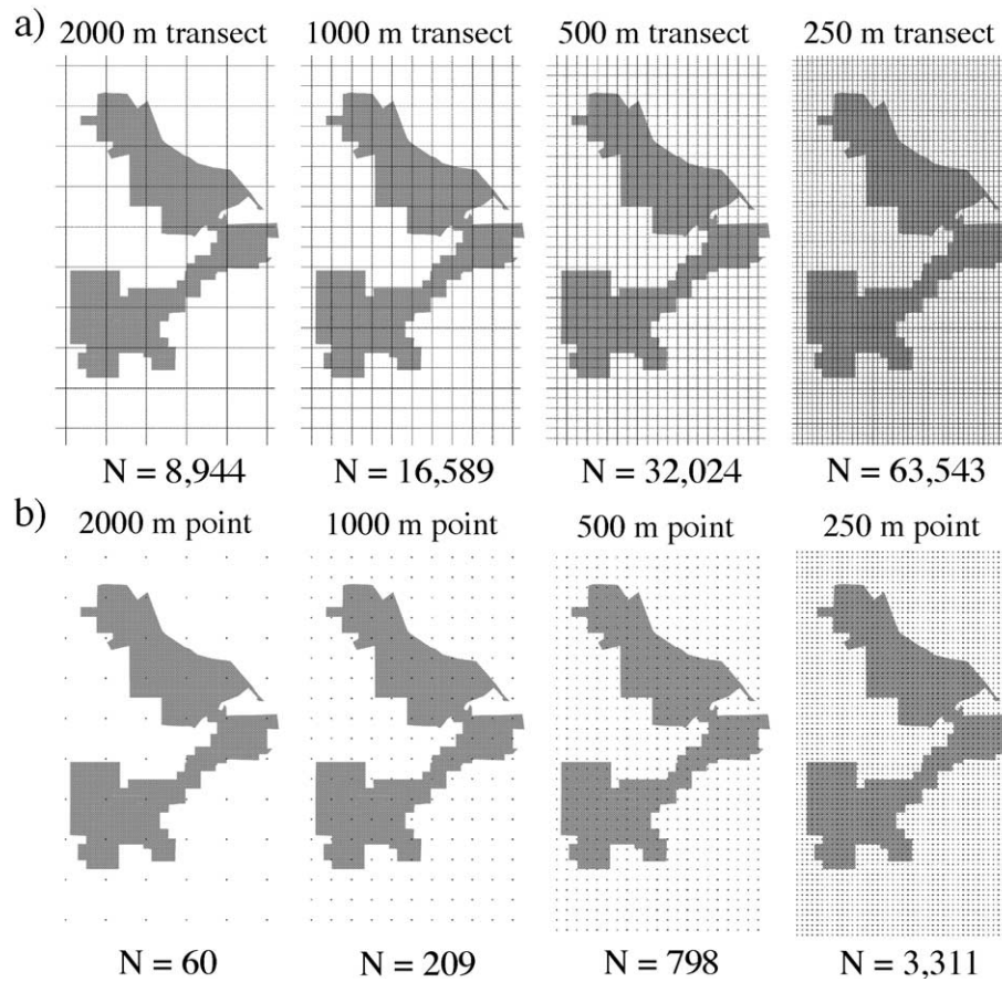
Fig. 2. (a) Transect and (b) Point sampling strategies tested and data volume of each sample dataset. The McDonald–Dunn Research Forest is shown in the background (see Fig. 1) for a spatial frame of reference.
