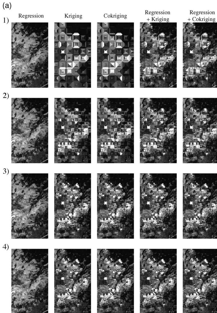
Fig. 8. (a) Estimated height maps from the five models tested, for the four transect sampling strategies: (1) 2000, (2) 1000, (3) 500, (4) 250 m, and (b) for the four point sampling strategies: (1) 2000, (2) 1000, (3) 500, and (4) 250 m. Brightness values are scaled to height values as in Fig. 1.
