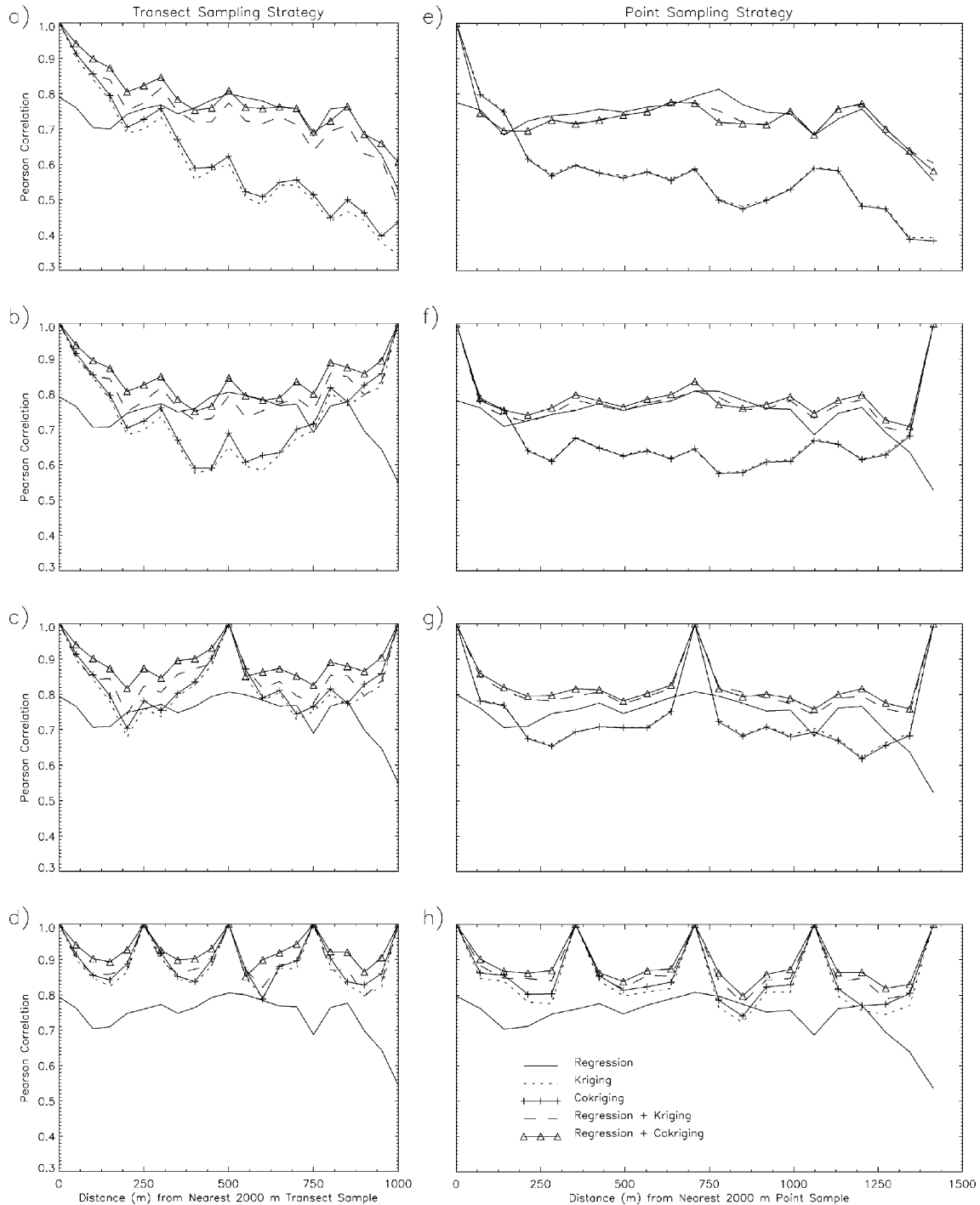
Fig. 7. Distance vs. Pearson's correlation coefficient for the eight sampling strategies tested: (a) 2000-m transect, (b) 1000-m transect, (c) 500-m transect, (d) 250-m transect, (e) 2000-m point, (f) 1000-m point, (g) 500-m point, and (h) 250-m point. The validation points are farther from the nearest point sample location than from the nearest transect sample location by a factor of \sqrt{2} . The graphed value at each distance is based on n=180 points, except n=60 at 0 m, and n=45 at 1000 (plots a–d) or 1414 m (plots e–h). Perfect correlations result in the spatial and integrated models where the validation and sample data locations intersect. Locations of the plotted values ( N=3525 ) are shown in Fig. 3.
