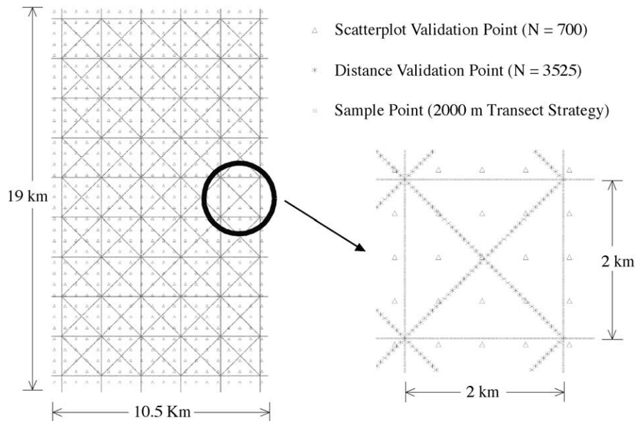
Fig. 3. Validation point locations. A grid of points representing the whole study area, but excluding any samples used for modeling, was systematically sampled to produce scatterplots of measured vs. estimated height ( \Delta ). Separate validation points were systematically sampled to evaluate the height estimates as a function of distance from sample locations (*). Sample points for the 2000-m transect sampling strategy are shown in the background (see Fig. 2) for a spatial frame of reference ( \blacksquare ).
