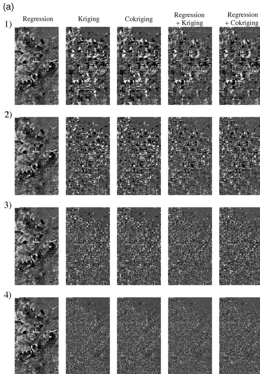
Fig. 9. (a) Estimated height error maps from the five models tested, for the four transect sampling strategies: (1) 2000, (2) 1000, (3) 500, and (4) 250 m, and (b) for the four point sampling strategies: (1) 2000, (2) 1000, (3) 500, and (4) 250 m. Bright areas are overestimates while dark areas are underestimates; see Table 3 for error magnitudes.
