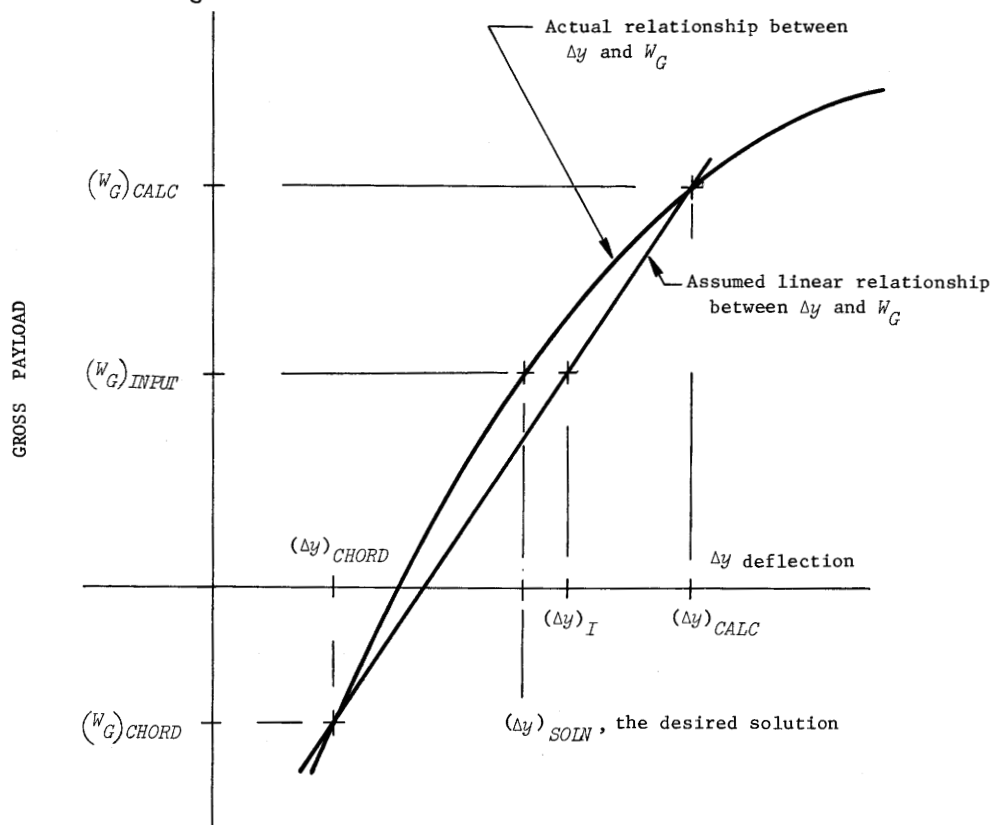
Figure 3.— \Delta y - W_G relationship.
