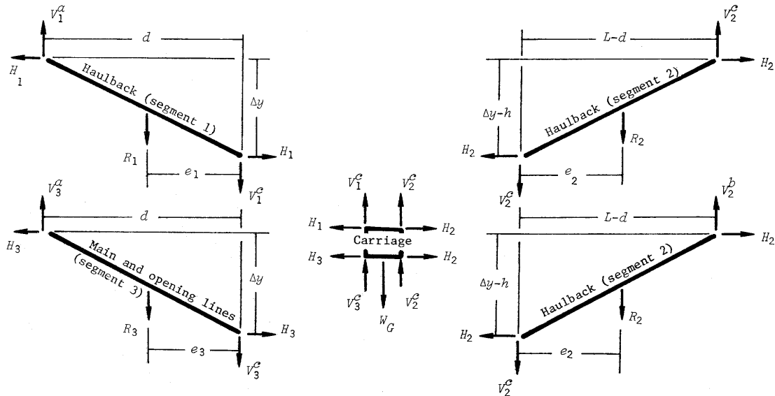
Figure 2.—Force balance formulation.
