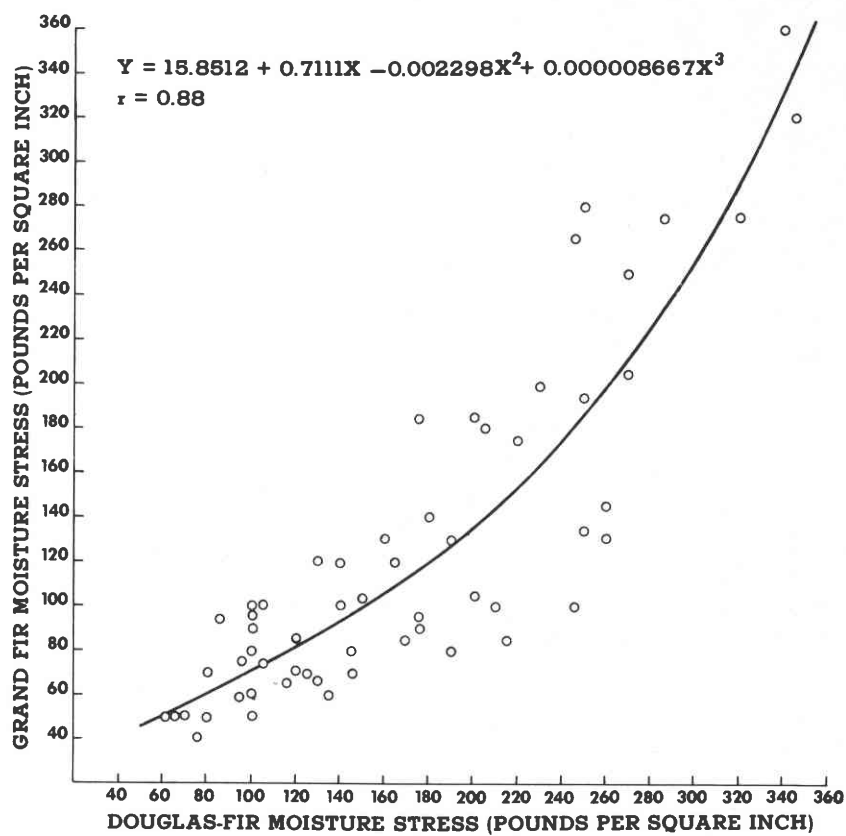
Figure 3.—Moisture stress regression for grand fir-Douglas-fir.
