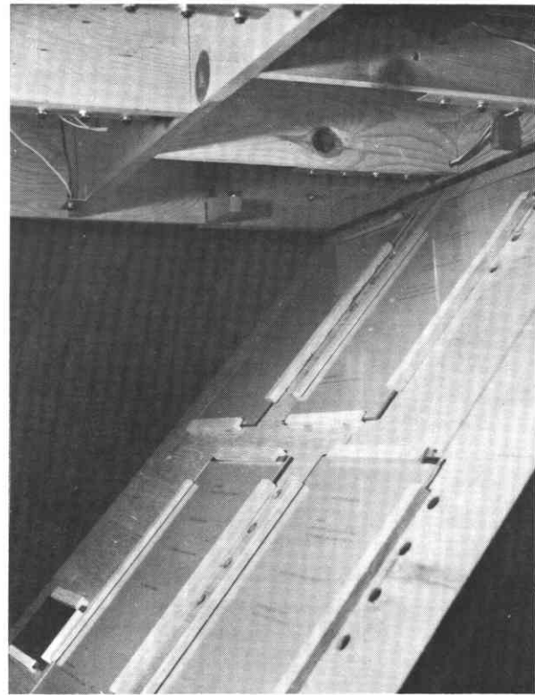
Figure 3.--Construction detail for the recording quizboard: (A) Counters and the wiring board for defining which buttons operate which counters. Each group of four plugs includes a green plug for correct answer and three red plugs for incorrect answers. (B) Each answer panel contains a "sandwich" of tracing paper and sheets of acrylic plastic. (C) The removable quizboard face permits answer panels to be quickly changed. (D) Each panel fits over a box with lights and reflectors for illumination.
