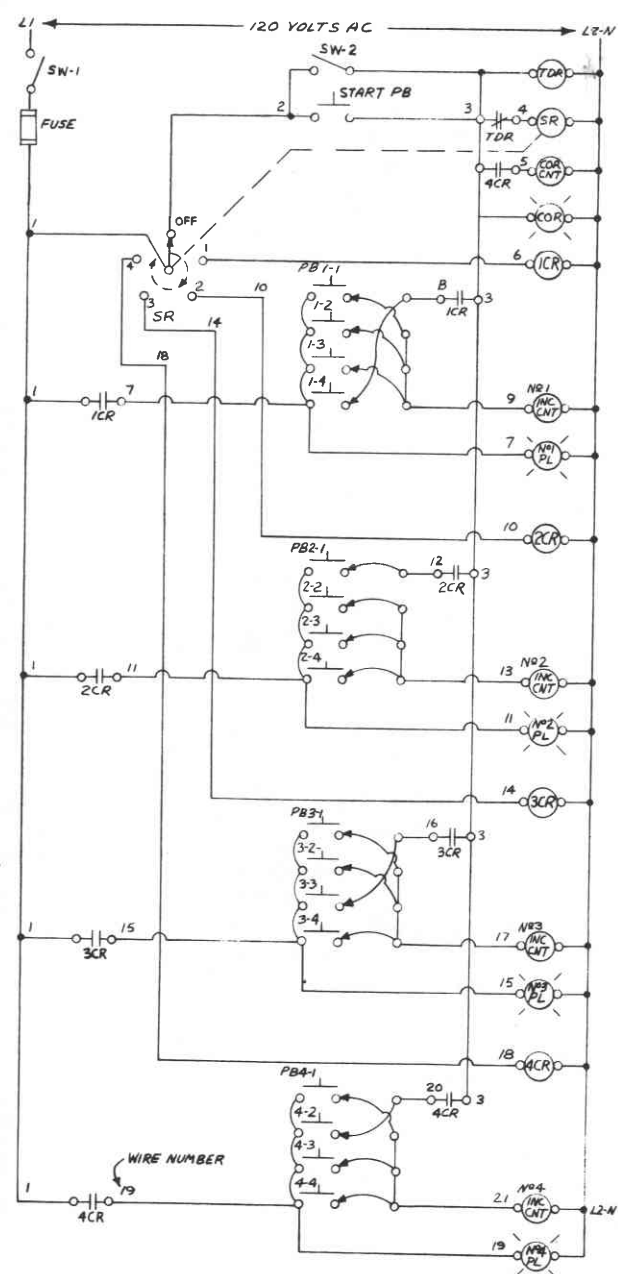
WIRING DIAGRAM
