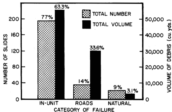
Figure 6.--Graph showing number of slope failures and estimated volumes of debris released by land-use category.
