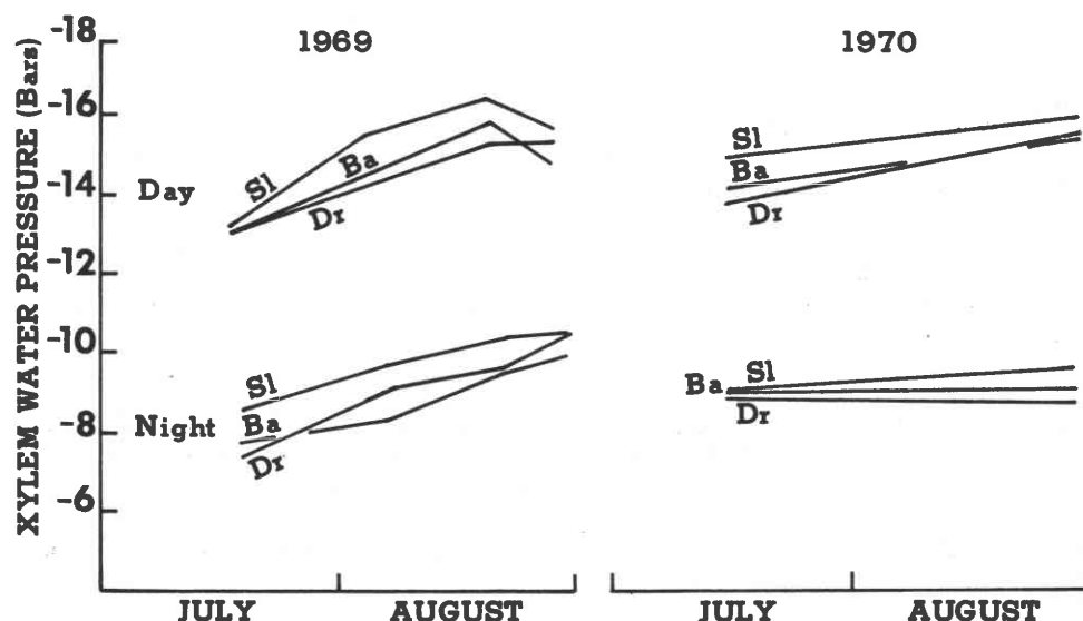
Figure 8.—Seasonal trend of moisture stress in lodgepole pine on three different sites (Sl—slopes, Dr—drainages, Ba—basins).
