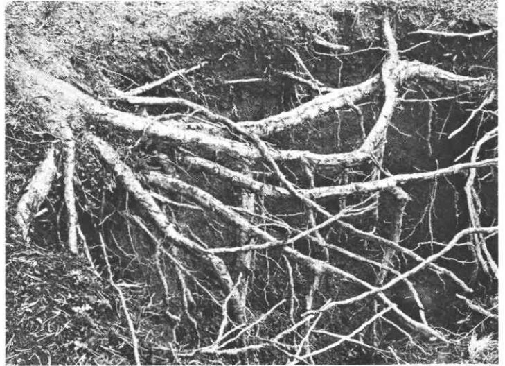
Figure 4.—Excavated roots of lodgepole pine showing: A, Shallow rooting on infested basin sites; and B, rooting in uninfested drainage sites.
