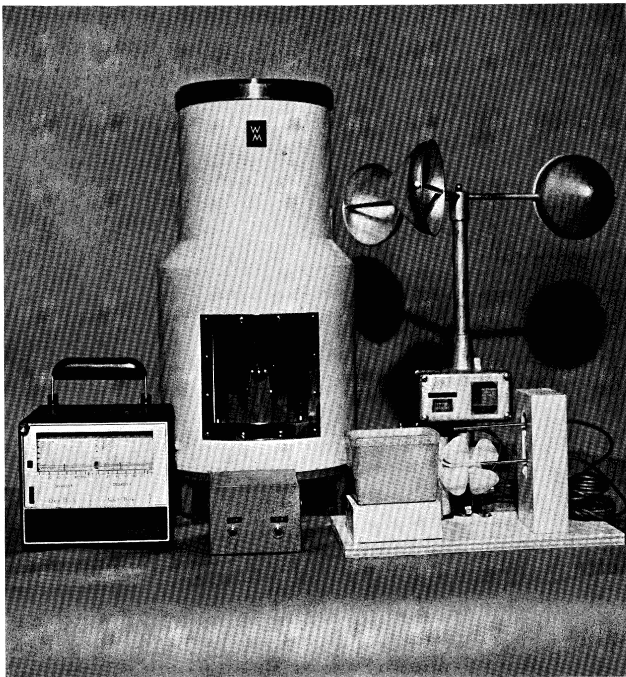
Figure 1.--Components of the recording weather station. Front row, left to right: recorder, "battery saver," psychrometer. Back row: tipping bucket rain gage, anemometer.
