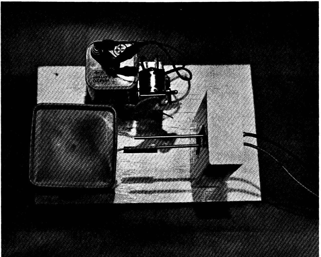
Figure 2.--Thermistor psychrometer used in the recording weather station.
