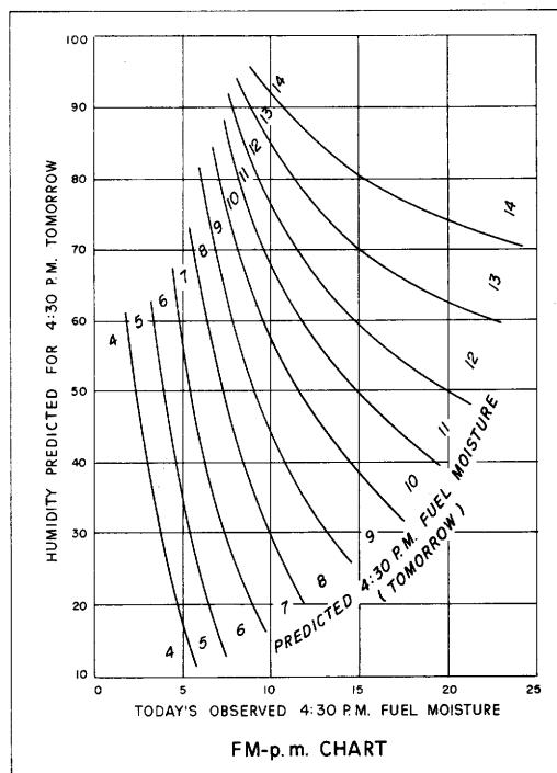
Figure 2.--Fuel-moisture estimation aids for a sample peak station.
