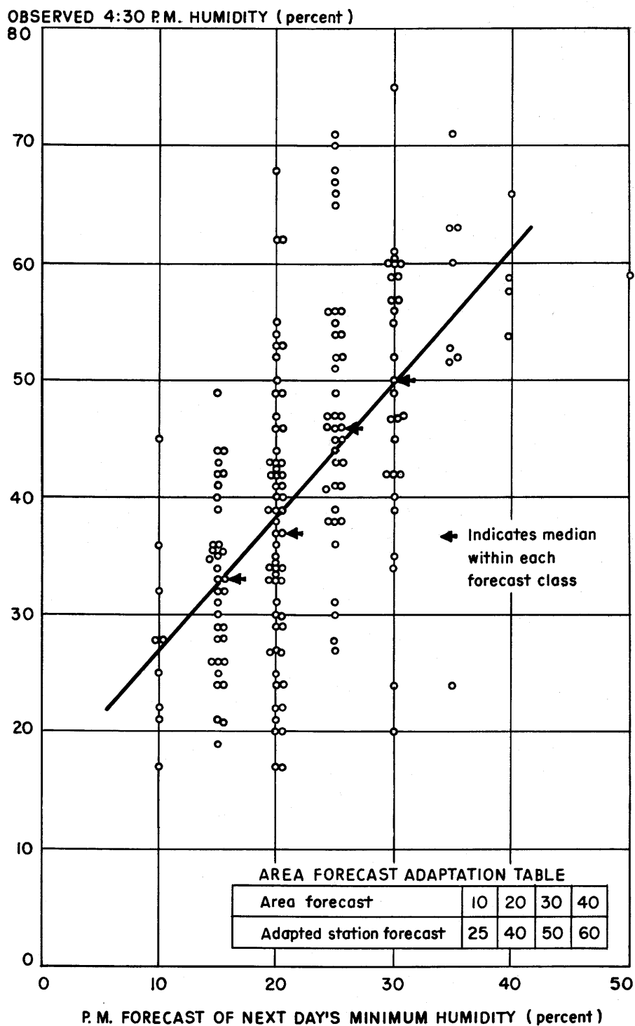
Figure 1.--Example of humidity forecast adaptation aid and worksheet.
