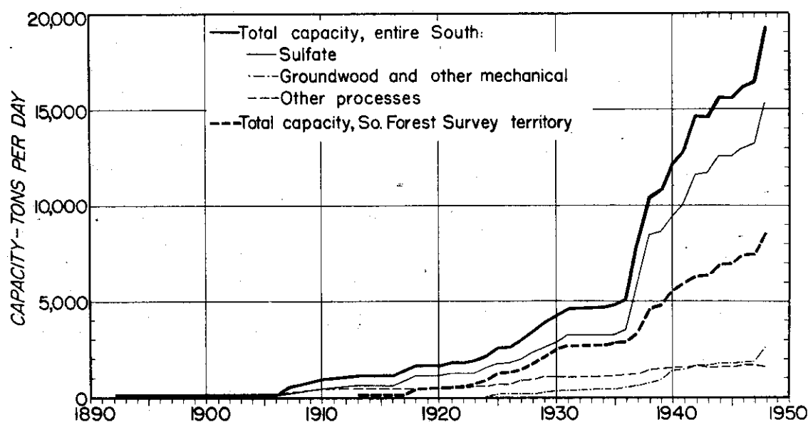
Figure 2.--Pulp-mill capacity in the South, 1892-1948.
