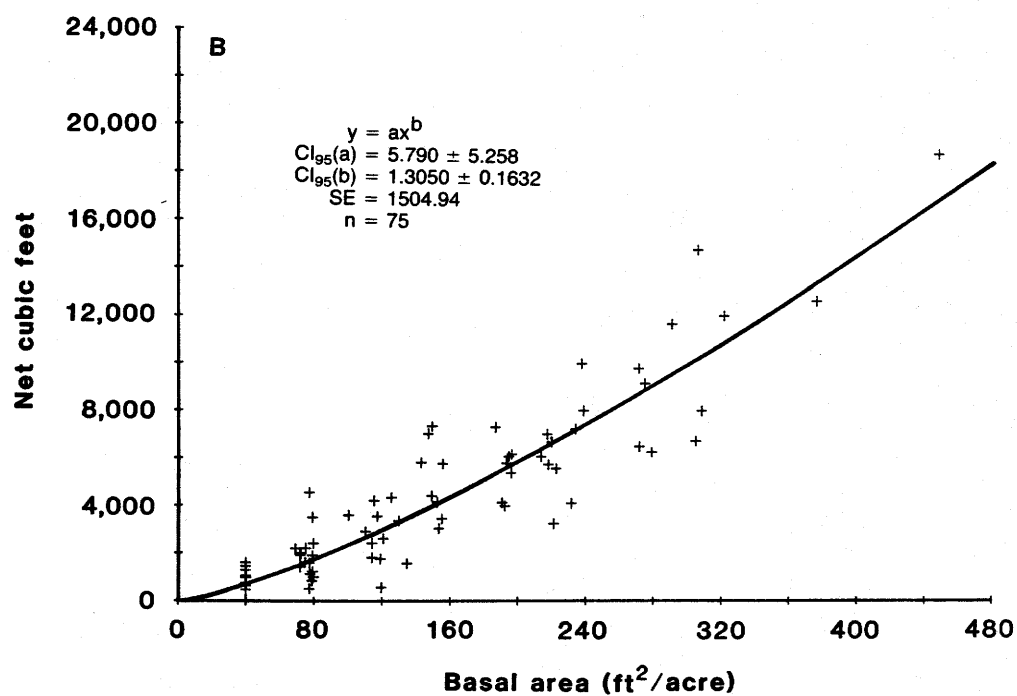
Figure 8.—Regressions of (A) gross cubic foot volume per acre and (B) net cubic foot volume per acre of western hemlock (species 263) over basal area per acre for the KPC sale.
