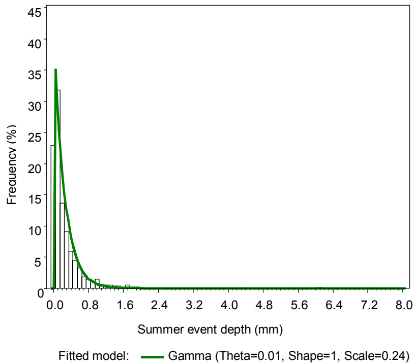
Figure 2-15. Frequency distribution of warm-season event depth fitted with gamma probability distribution function ( p -value =0.042).
