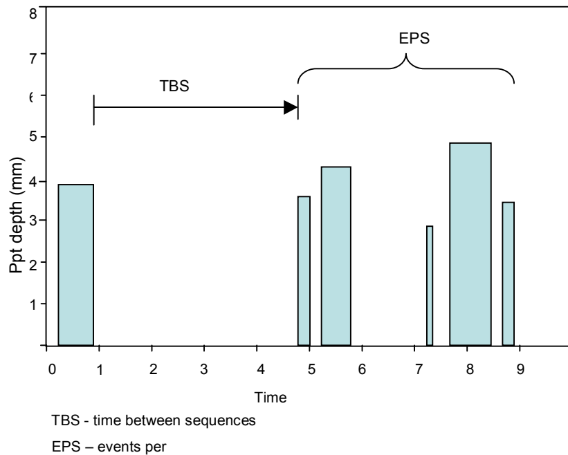
Figure 2-3a. Cold-season model variables for storm sequences.
