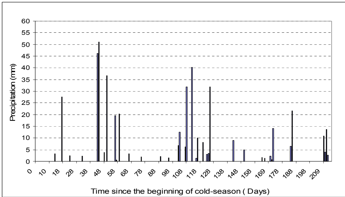
Figure 3-13. Simulated daily precipitation vs. time for one cold-season.
