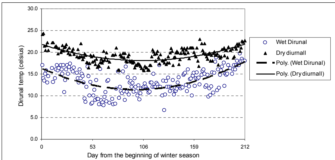
Figure 2-30. Graph of average cold-season diurnal temperature variations for dry and wet days fit the second degree parabolic functions.
