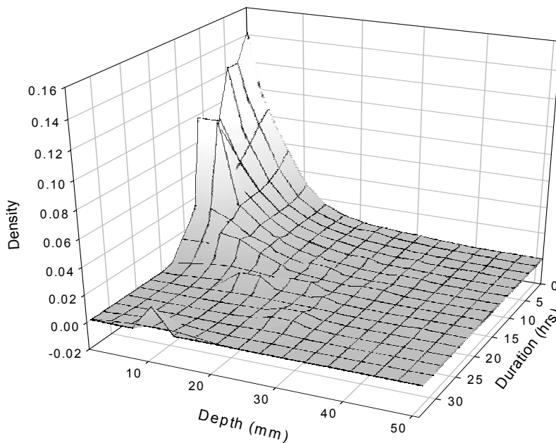
Figure 2-17. Bivariate probability density of observed warm-season precipitation depth.
