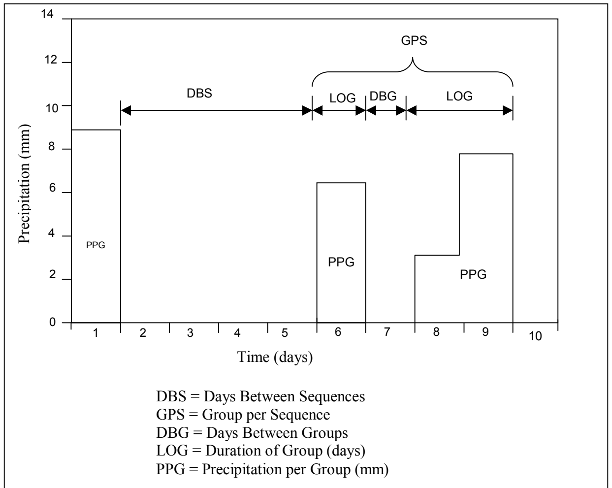
Figure 2-1. Winter precipitation model variables as described in Duckstein et al., (1975).
