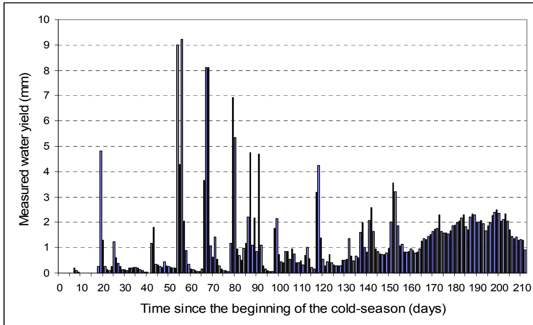
Figure 3-15. Twenty year average measured daily stream flow for the cold-season.
