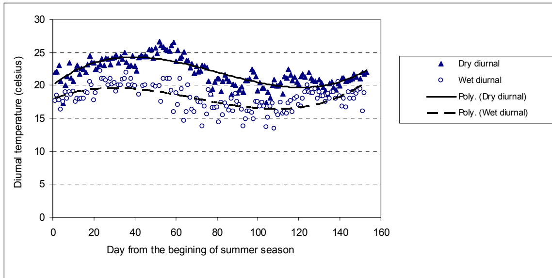
Figure 2-32. Graph of average warm-season diurnal temperatures variation for dry and wet days fitted with three degree parabolic functions
