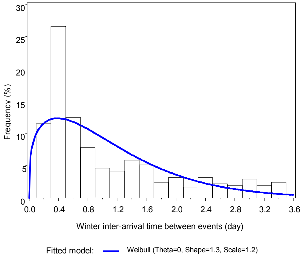
Figure 2-5. Frequency distribution of interarrival time between cold-season events fitted with Weibull probability distribution function ( p -value = 0.01).
