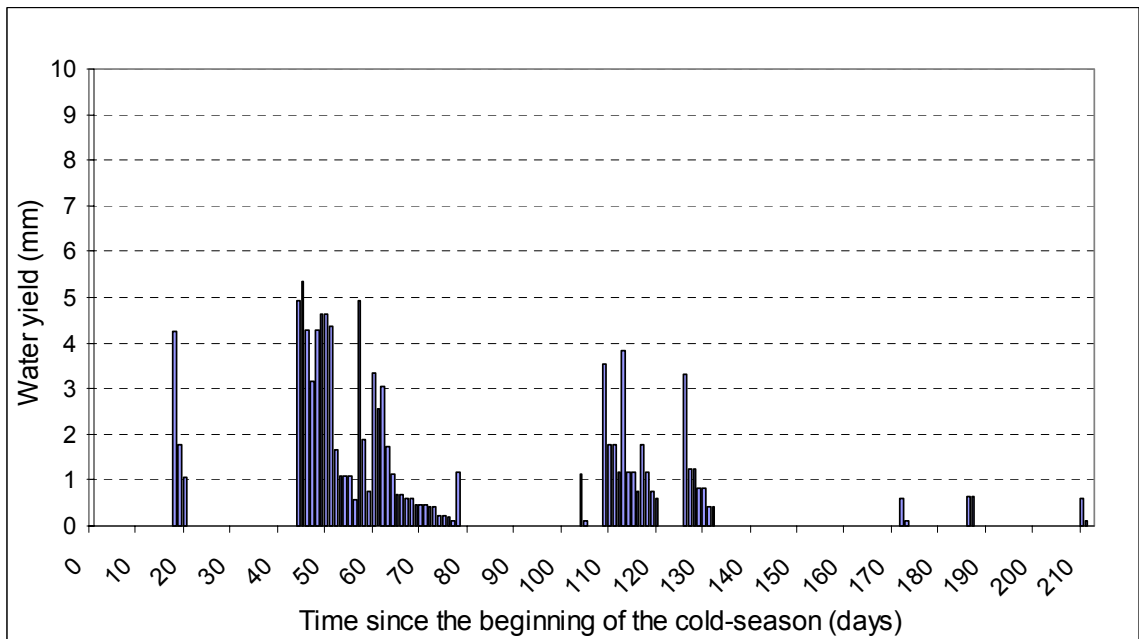
Figure 3-14. Simulated daily water yield vs. time for one cold-season.
