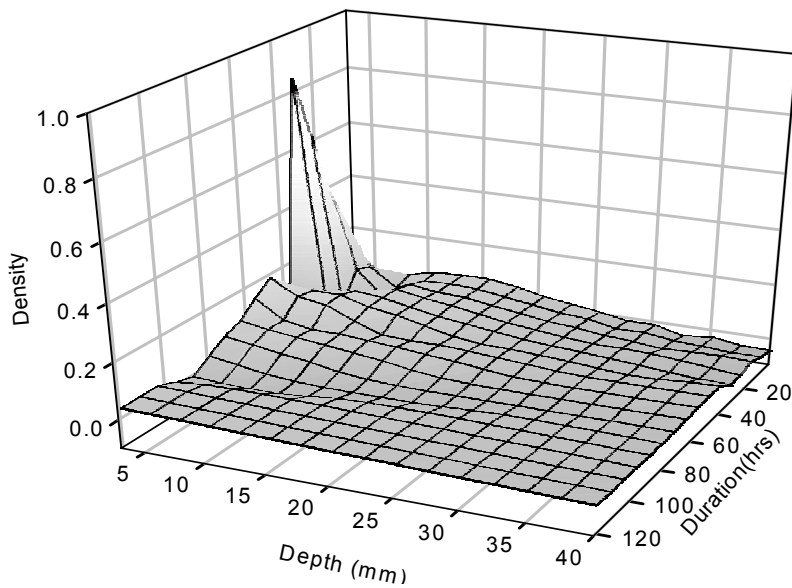
Figure 2-11. Bivariate probability density of simulated cold-season precipitation depth.
