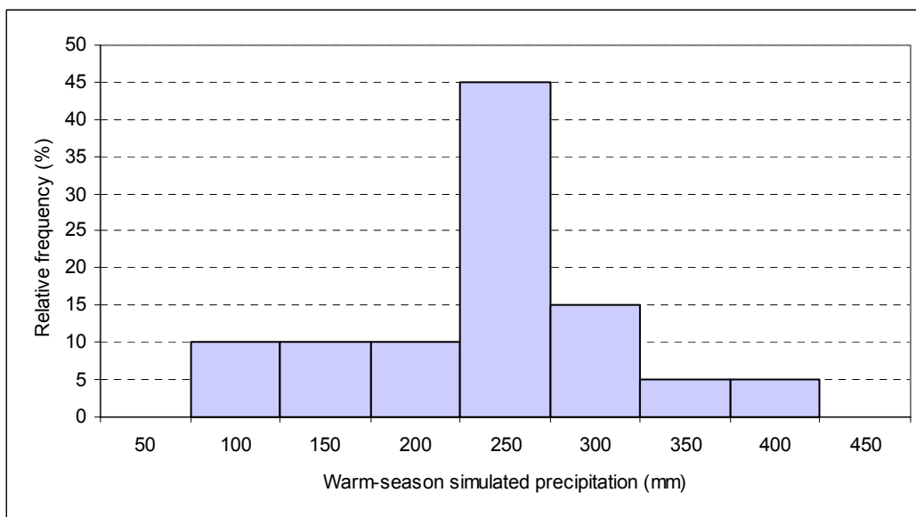
Figure 2-20. Relative frequency of simulated warm-season precipitation. (N = 20 years).
