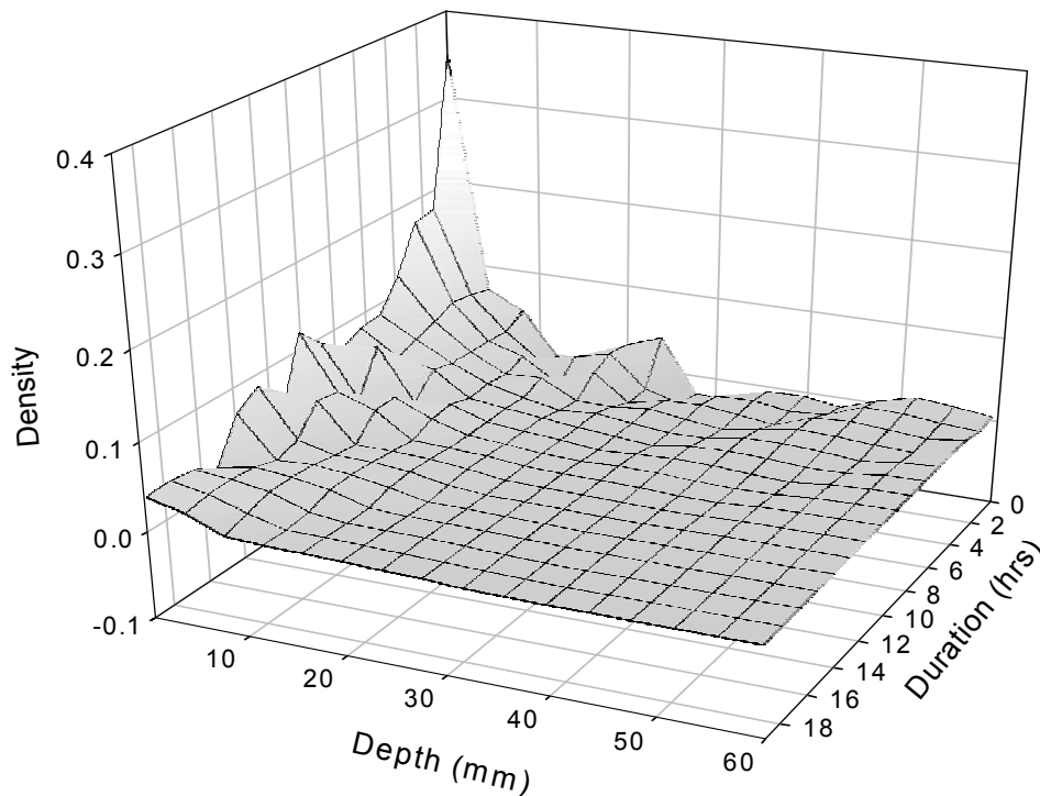
Figure 2-18. Bivariate probability density of simulated warm-season precipitation depth.
