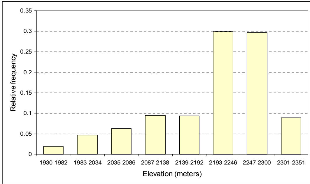
Figure 3-5. Relative frequency histogram of elevation.
