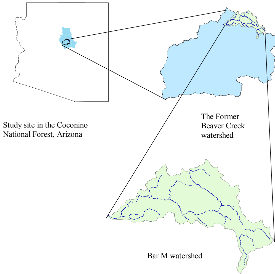
Figure 1-1. Location of Mar M watershed in the former Beaver Creek experimental watershed.
