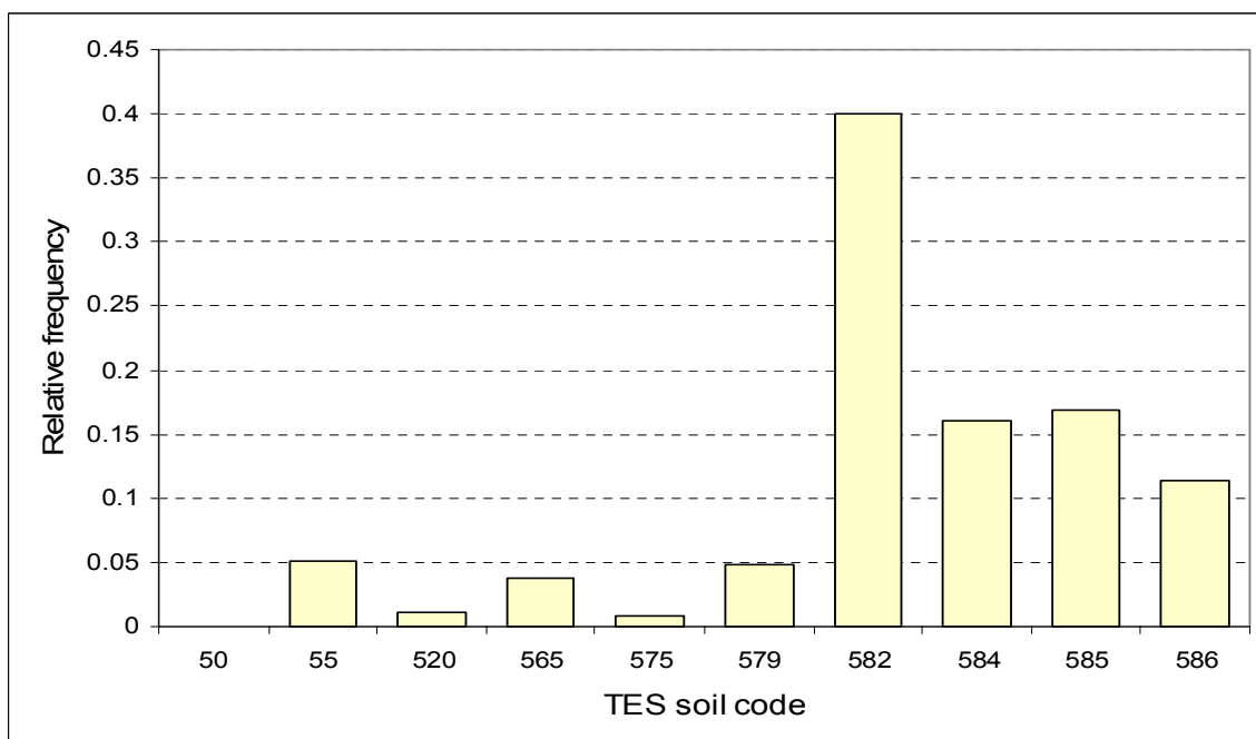
Figure 3-8. Relative frequency histogram of soil type.
