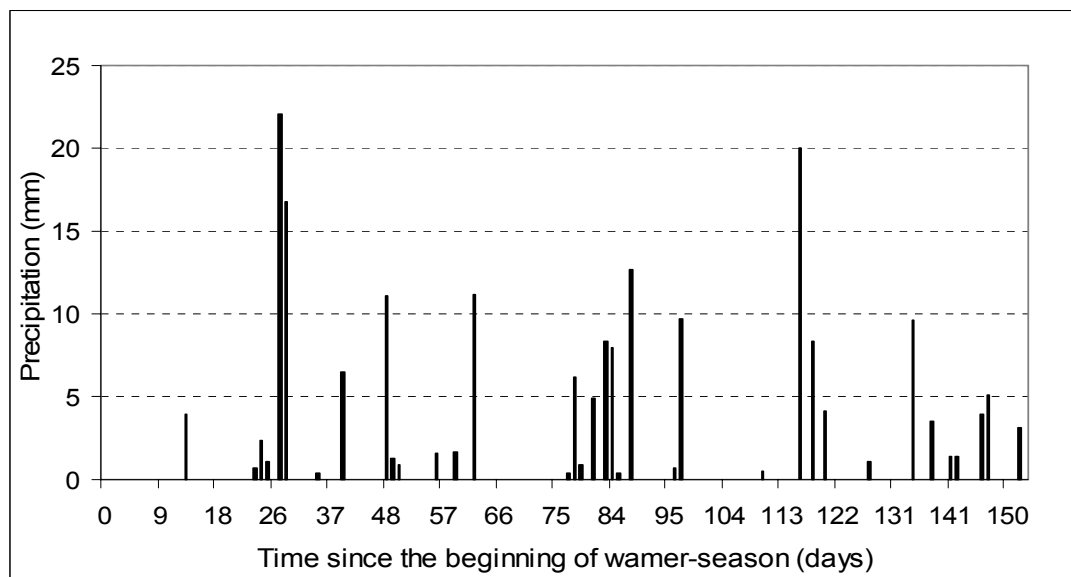
Figure 3-17. Simulated daily precipitation vs. time for one warm-season.
