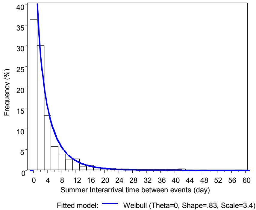
Figure 2-14. Frequency distribution of interarrival time between warm-season events fitted with Weibull probability distribution function ( p -value =0.01).
