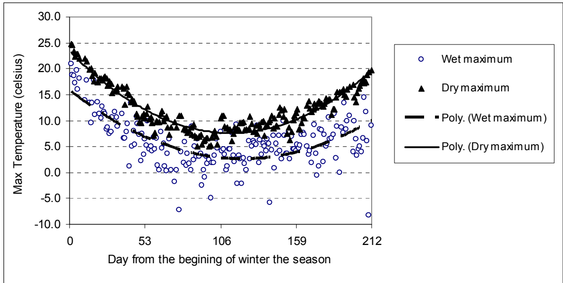
Figure 2-29. Graph of average cold-season daily maximum temperatures for dry and wet days fit the second degree parabolic functions.
