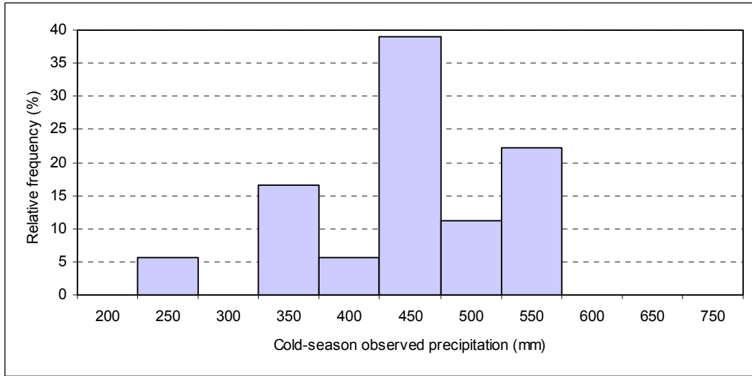
Figure 2-12. Relative frequency of measured cold-season precipitation. N = 20 years.
