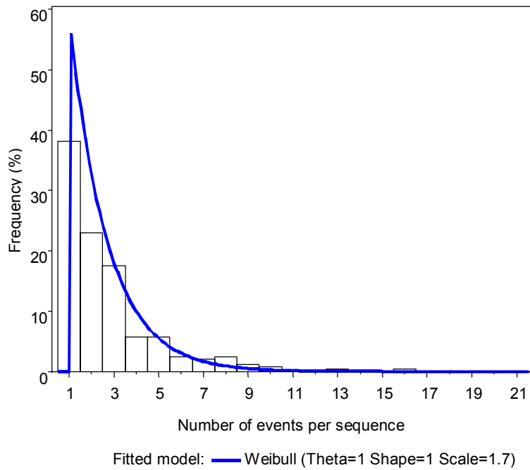
Figure 2-6. Frequency distribution of number of events per sequence fitted with Weibull probability distribution function ( p -value = 0.01).
