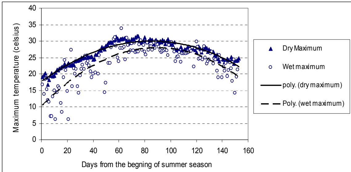
Figure 2-31. Graph of average warm-season maximum temperatures for dry and wet days fitted with second degree parabolic functions.
