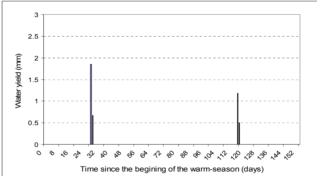
Figure 3-18. Simulated daily water yield vs. time for one warm-season.
