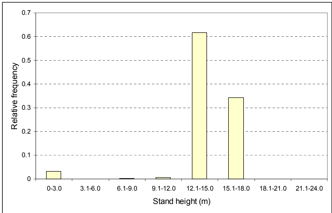
Figure 3-12. Relative frequency histogram of stand height.
