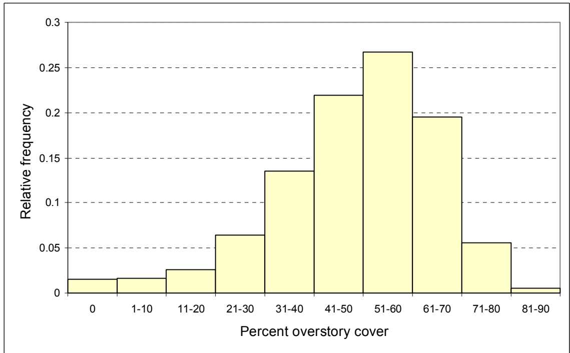
Figure 3-10. Relative frequency histogram of the overstory cover
