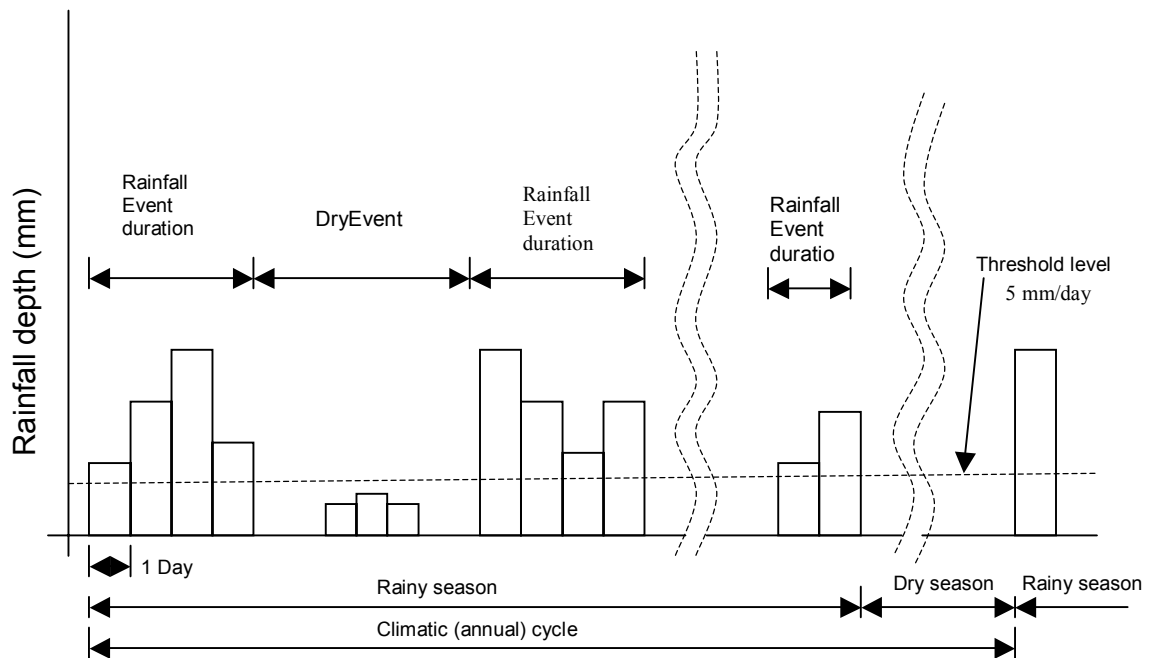
Figure 2-2. Summer precipitation model variables (Bogardi et al., 1988).
