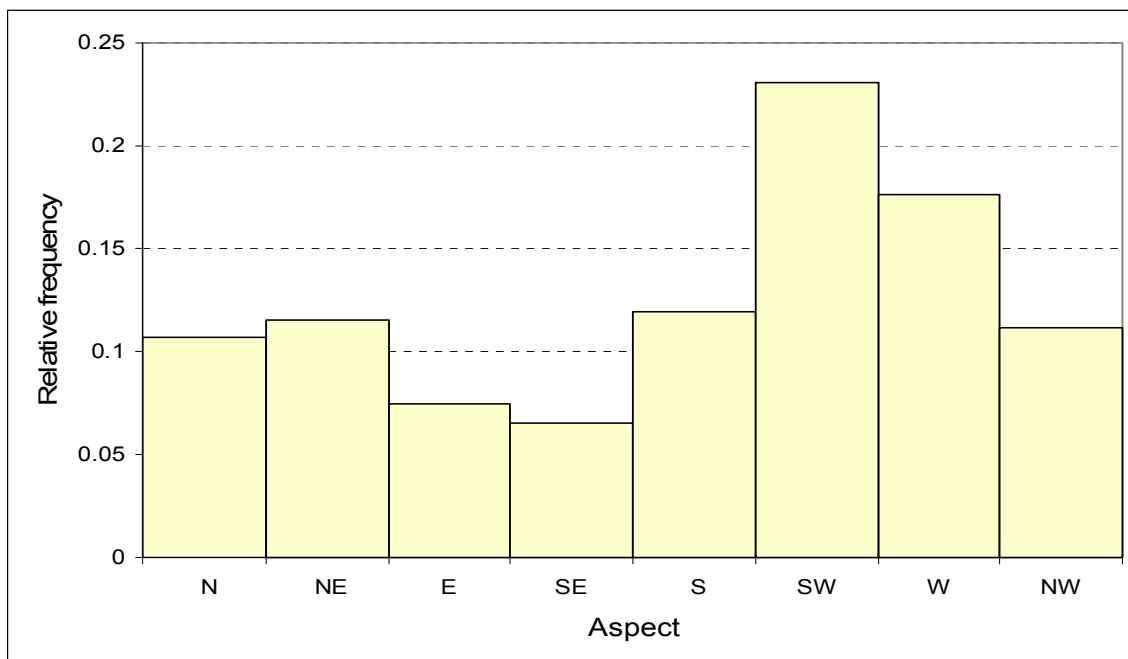
Figure 3-7. Relative frequency histogram of aspect.
