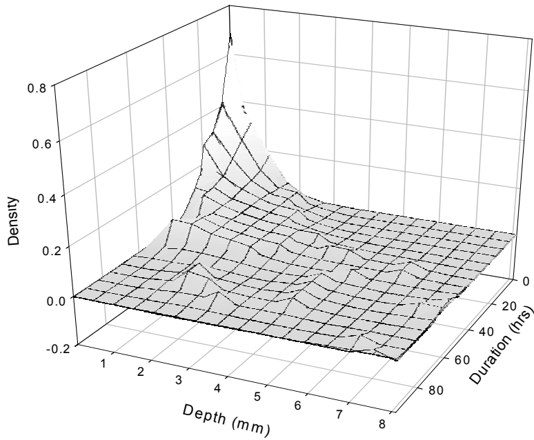
Figure 2-10. Bivariate probability density of observed cold-season precipitation depth.
