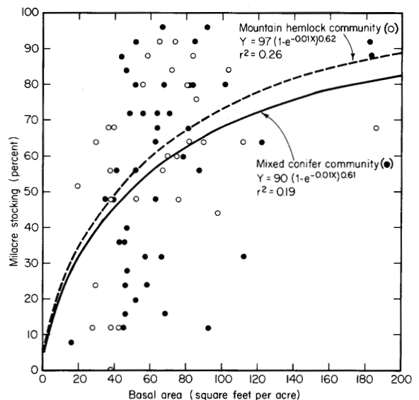
Figure 7.--Relationship between basal area and milacre stocking of natural regeneration in the mountain hemlock and mixed conifer plant communities in the Cascade Range of eastern Oregon.
