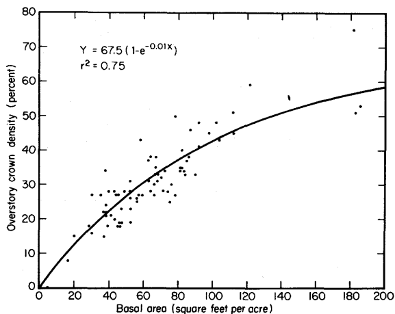
Figure 5.--Relationship between basal area and crown density of residual overstory for all shelterwood plots in both mountain hemlock and mixed conifer plant communities in the eastern Cascade Range.
