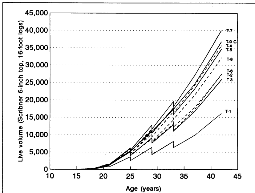
Figure 14—Board-foot volume by age for fixed, increasing, and decreasing treatments.
