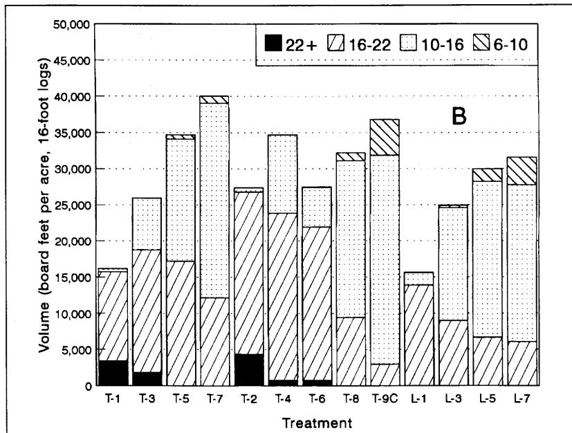
Figure 17—Standing volume at age 42 by tree diameter classes in inches for (A) cubic feet per acre and (B) board feet per acre (Scribner, 16-foot logs).
