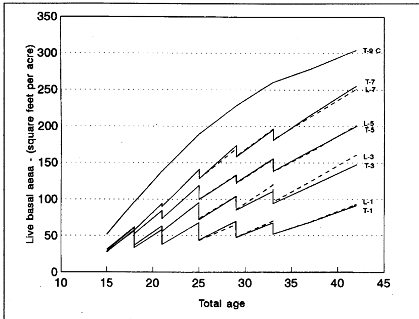
Figure 9—Live basal area by age for fixed early (T) and late (L) thinning treatments.
