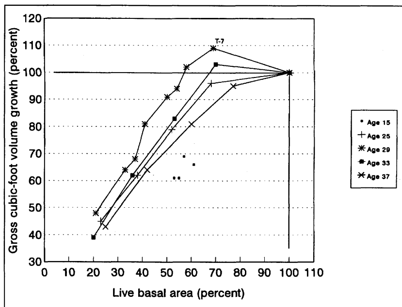
Figure 22—Volume growth to basal area growing stock relations of treatment averages expressed as percentages of unthinned control by age of stand.
