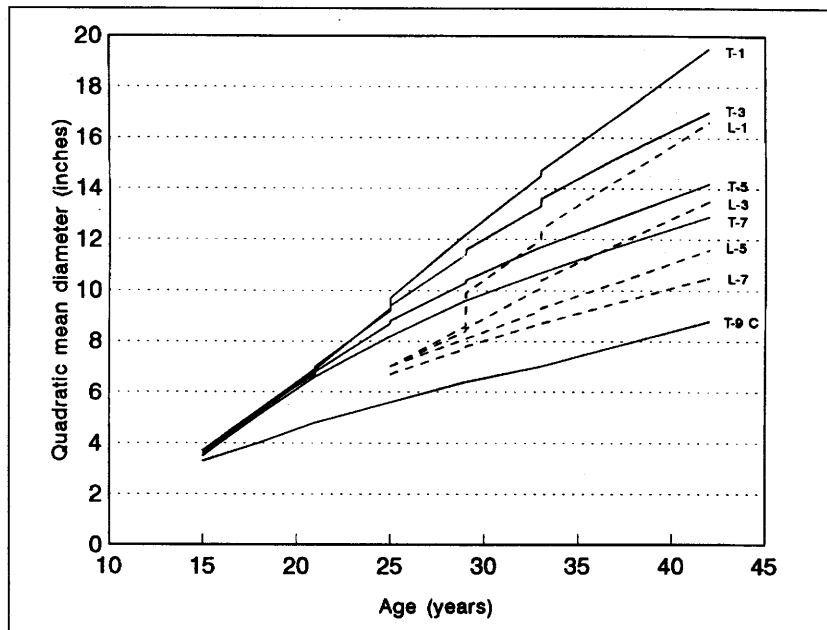
Figure 7—Quadratic mean diameter by age for fixed early (T) and late (L) treatments.
