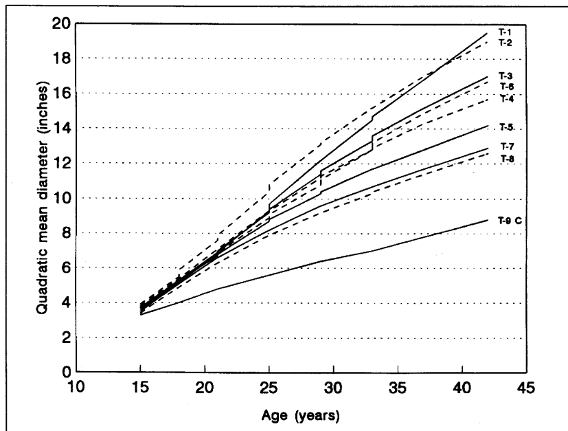
Figure 8—Quadratic mean diameter by age for increasing and decreasing treatments.
