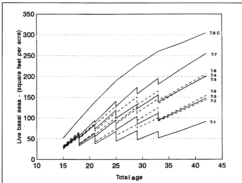
Figure 10—Live basal area by age for increasing and decreasing treatments.
