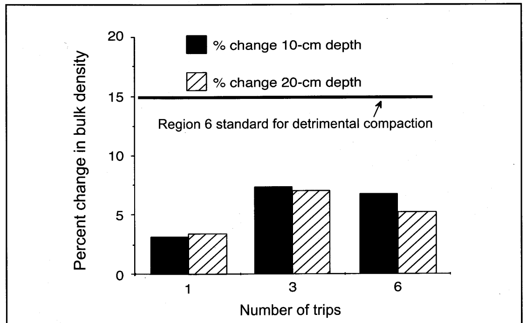
Figure 2—Percentage of increase in soil bulk densities at 10-cm and 20-cm soil depths after zero, one, three, and six trips with a John Deere 450E in southwestern Oregon.
