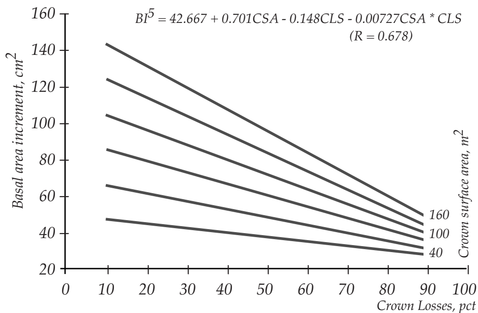
Figure 3 — Influence of qualitative and quantitative composite crown indicators on tree increment.
