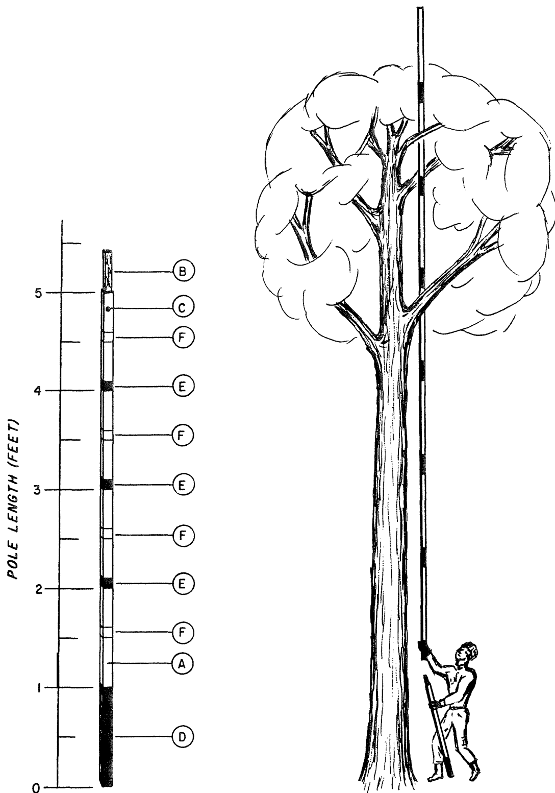
Figure 1. --Construction features of sectional aluminum poles: A , 1- by 1-inch square aluminum tubing, 5 feet long; B , 7/8- by 7/8- by 8-inch treated hickory peg; C , sheet-metal screw; D , black plastic tape; E , red plastic tape; F , yellow plastic tape.
