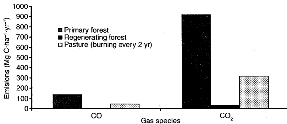
FIG. 5. Emissions of CO and CO 2 arising from burning primary forest slash, regenerating forest slash, and pastures for the extent of the Jamari, Rondônia, study area (94 370 ha) during the study period (1984–1992). Pasture emissions include pastures burned between 1984 and 1986 and modeled pastures reburned on a frequency of 2 yr for the 1986–1992 period.
