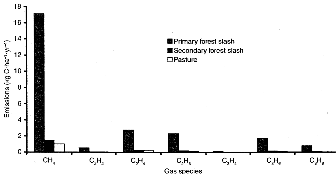
FIG. 2. Emissions of CH 4 and trace gases arising from fires in primary forest slash, regenerating forest slash, and pastures for the extent of the Jamari, Rondônia, study area (1984–1986).
