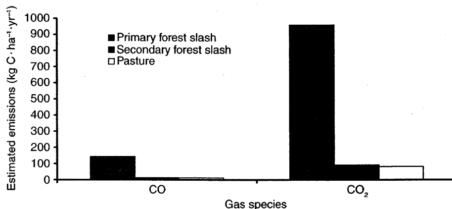
FIG. 1. Estimated emissions of CO and CO 2 from fires in primary forest slash, regenerating forest slash, and pastures for the extent of the Jamari, Rondônia, study area (1984–1986).
