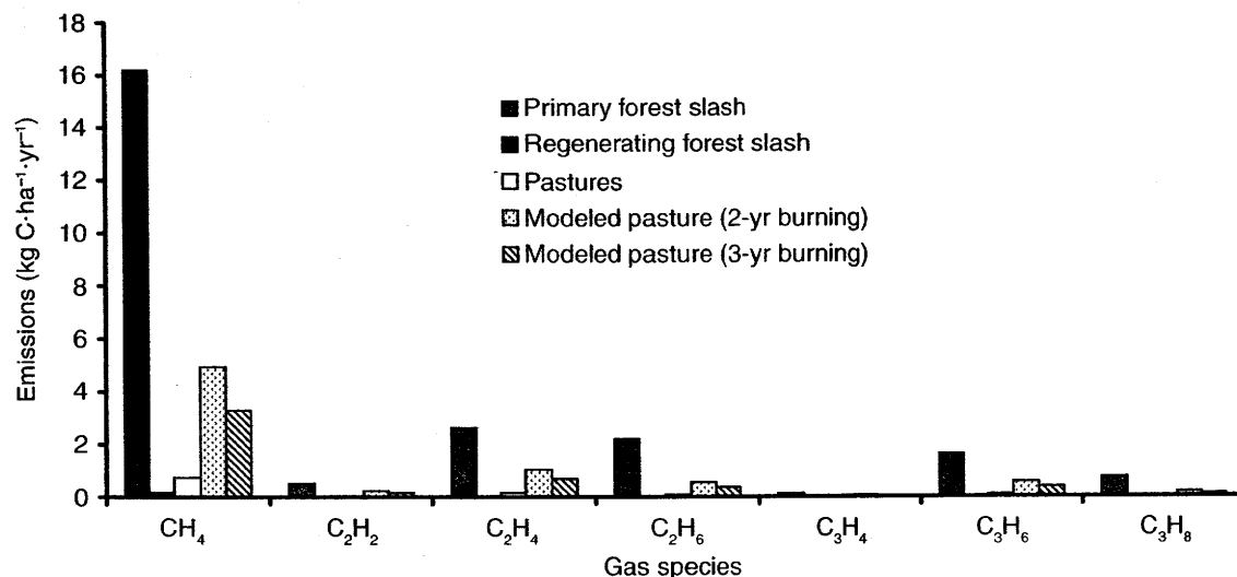
FIG. 4. Emissions of trace gases from burning primary forest slash, regenerating forest slash, and pastures (burned once) for the extent of the Jamari, Rondônia, study area (1986–1992). Modeled pasture emissions include pastures reburned on a frequency of 2 or 3 yr during the study period.
