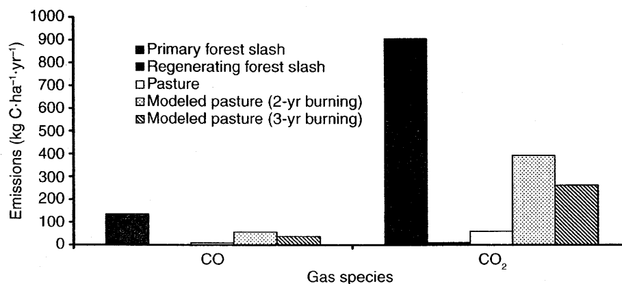
FIG. 3. Emissions of CO and CO 2 arising from burning primary forest slash, regenerating forest slash, and pastures (burned once) for the extent of the Jamari, Rondônia, study area (1986–1992). Modeled pasture emissions include pastures reburned on a frequency of 2 or 3 yr during the study period.
