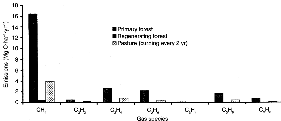
FIG. 6. Emissions of trace gases arising from burning primary forest slash, regenerating forest slash, and pastures for the extent of the Jamari, Rondônia, study area (94 370 ha) during the study period (1984–1992). Pasture emissions include pastures burned between 1984 and 1986 and modeled pastures reburned on a frequency of two years for the 1986–1992 period.
