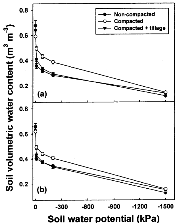
Fig. 4. Water retention curves for non-compacted, compacted, and compacted and tilled soil at the (a) 0- to 10-cm, and (b) the 10- to 20-cm depth at Fall River. Values are means \pm one standard error.
