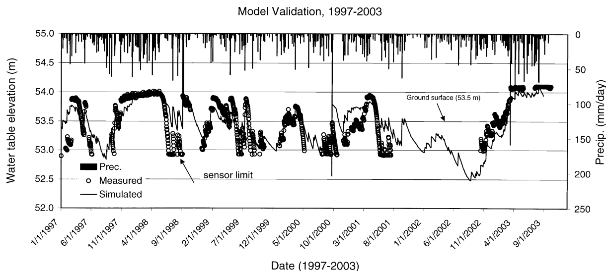
Figure 5. A seven-year model validation suggests that the wetland hydroperiod is mostly controlled by climate variability and that it can recover from extended drought rather quickly.
