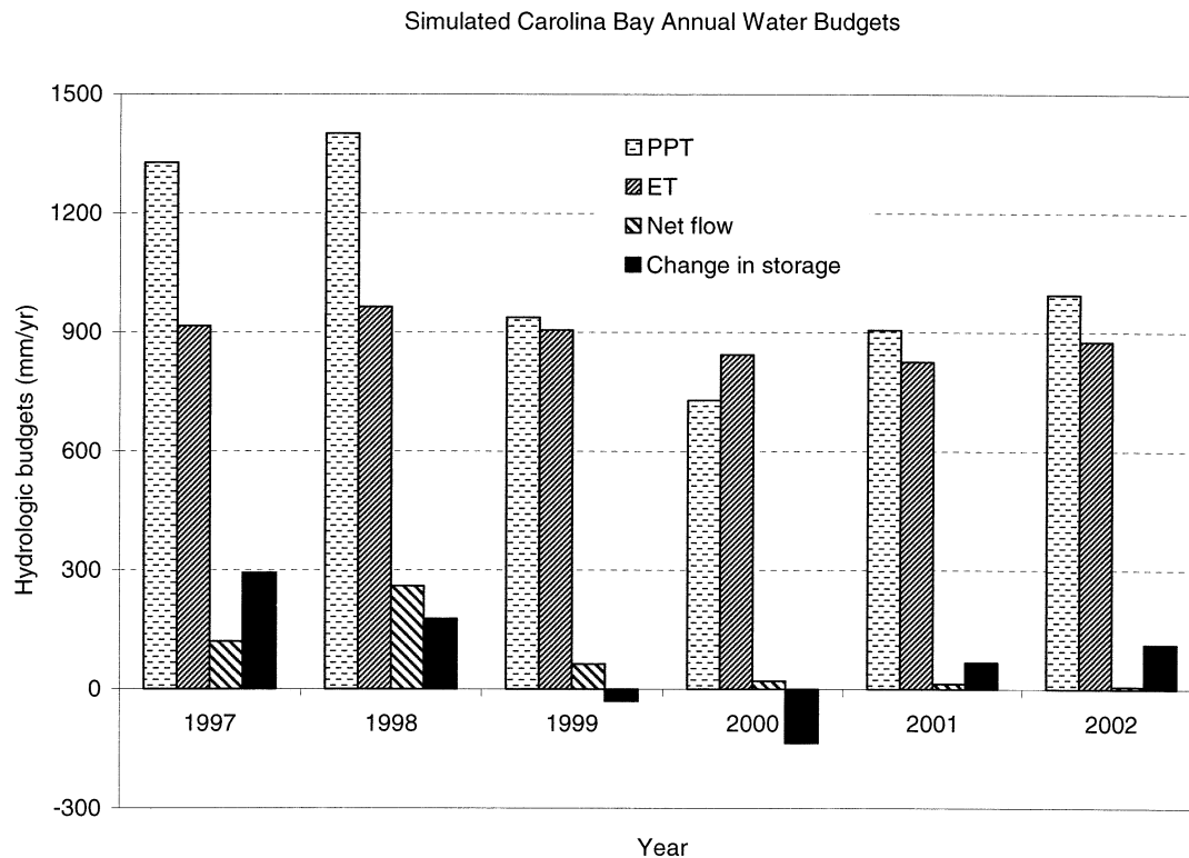
Figure 7. Simulated annual water budgets of the Chapel bay during 1997–2002 showing the water balance dominated by precipitation and evapotranspiration and ground-water flow most pronounced during wet years.
