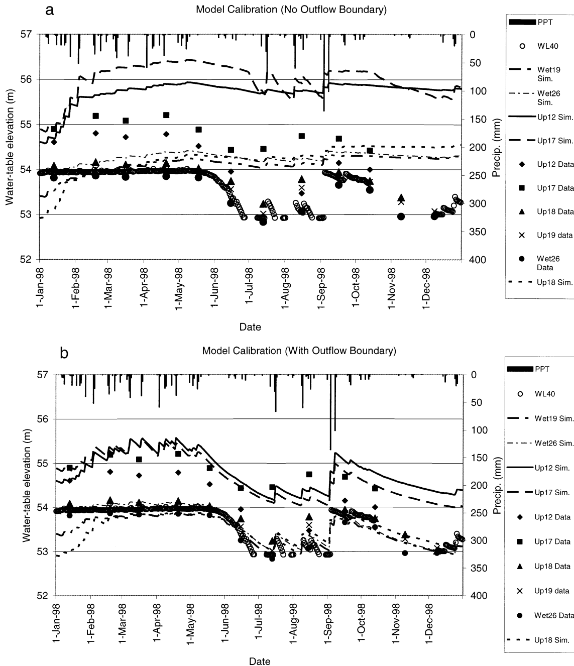
Figure 4. Model calibration using a) a no flow boundary and b) a fixed-head (54 m a.s.l.) boundary condition suggests that Chapel Bay is not hydrologically isolated from the surrounding upland and that lateral ground-water- surface-water interactions are common.
