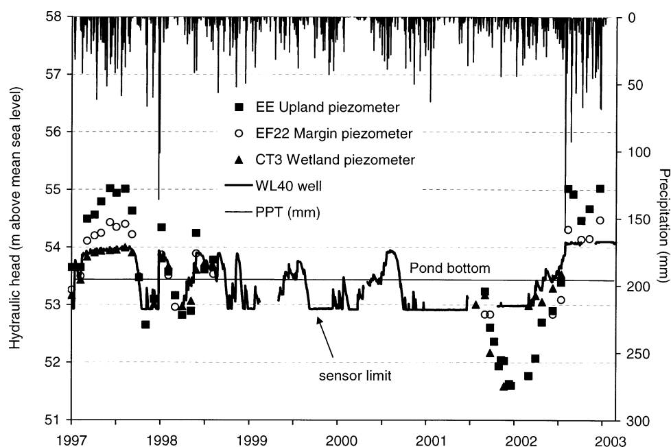
Figure 3. Measured water-table elevation (i.e., total hydraulic head) data at the upland, wetland-upland margin, and in the wetland indicates that the Chapel Bay is an unconfined aquifer system.
