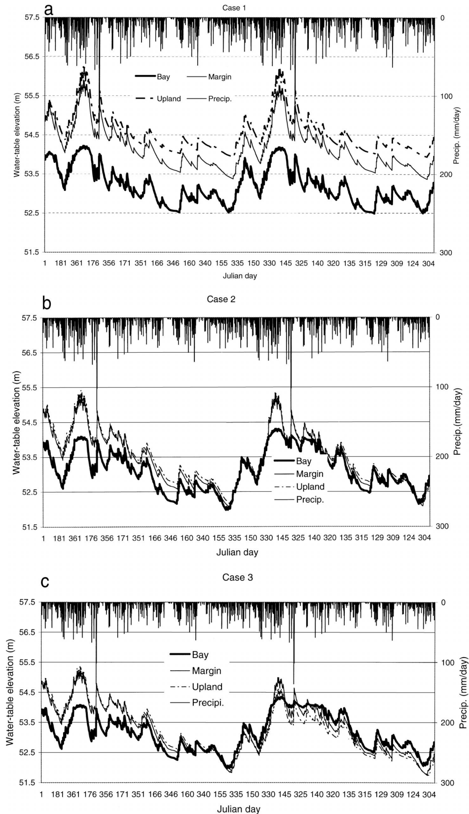
Figure 9. Comparison of water-table elevations (i.e., total hydraulic head) across the upland-wetland gradient for a) Case 1: Subsurface restricting layers parallel ground topography, b) Subsurface restricting layers are flat at 51 m elevation, and c) Case 3: reversed subsurface restricting layer to topographic gradient.
