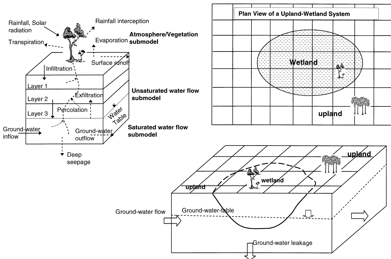
Figure 1. Sketch of the FLATWOODS model structure and hydrologic components.
