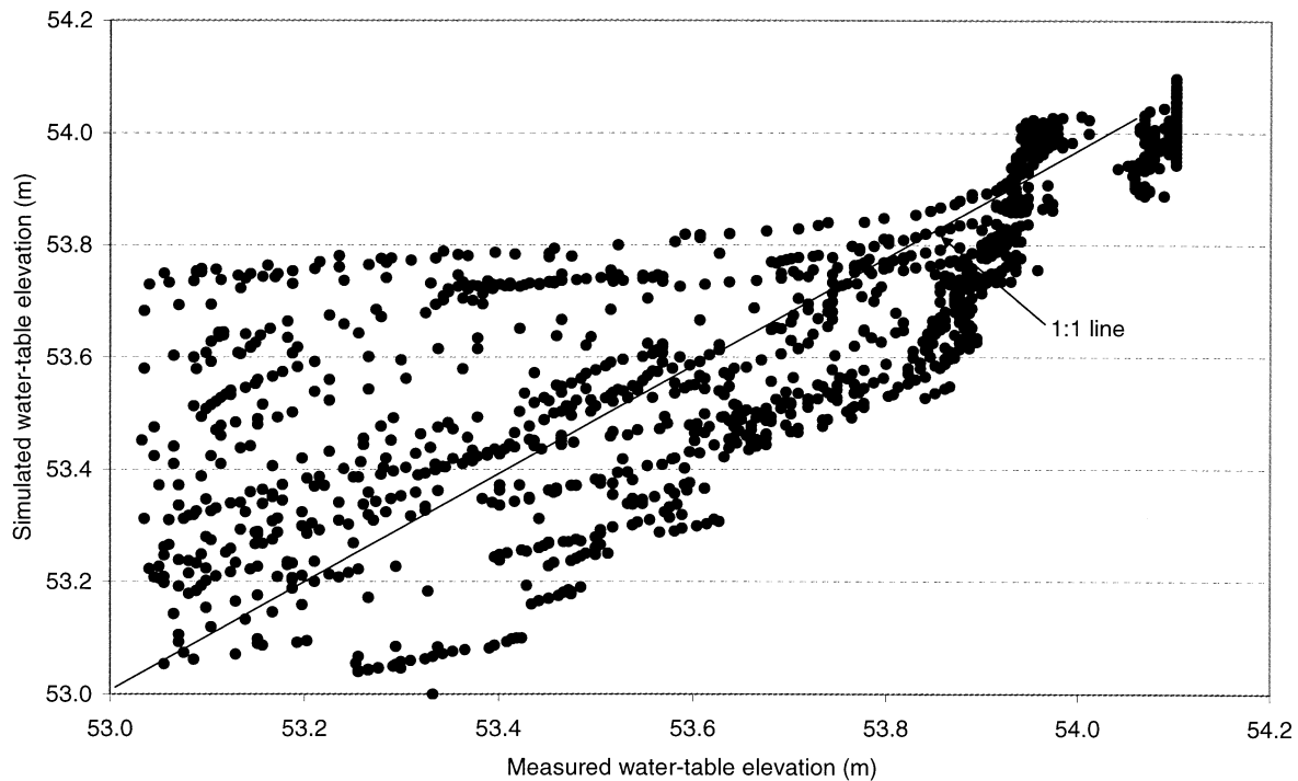
Figure 6. Comparison of simulated and measured water-table elevation (i.e., total hydraulic head) at Chapel Bay during the entire study period showing significant correlation but overestimation mostly during dry periods.
