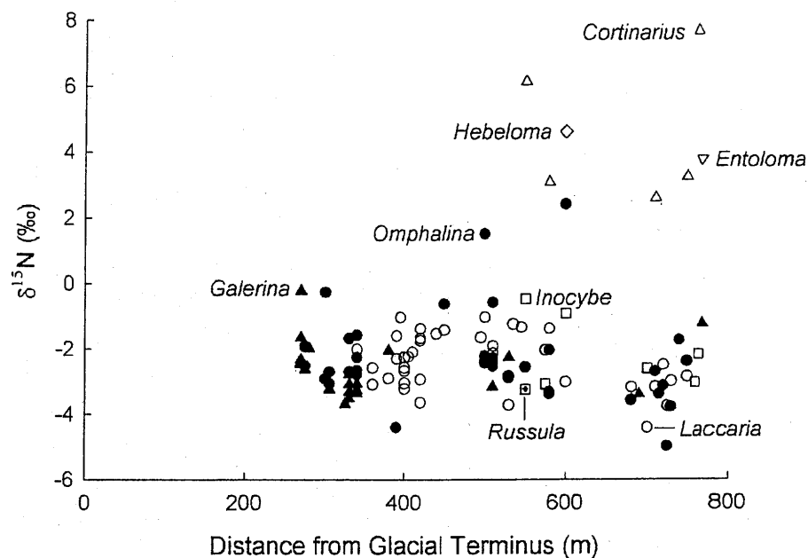
Fig. 3 \delta^{15}\text{N} patterns in fungi after glacial retreat at Lyman Glacier, Washington, USA. x-axis indicates distance from current glacial terminus, site ages range from 20 to 70 years (Jumpponen et al. 1998). Cortinarius tenebricus , Entoloma sp., Hebeloma sp., Inocybe lacera , Laccaria montana , and Russula fragilis are ectomycorrhizal fungi, whereas Galerina sp. and Omphalina obscurata are saprotrophic fungi. Clear symbols are for ectomycorrhizal taxa and filled symbols for saprotrophic taxa. Symbols for specific taxa are: Cortinarius , upright triangle; Entoloma , upside-down triangle; Hebeloma , diamond; Inocybe , square; Laccaria , circle; Russula , square with center cross; Galerina , upright filled triangle; and Omphalina , filled circle. Values for fungi represent single specimens
