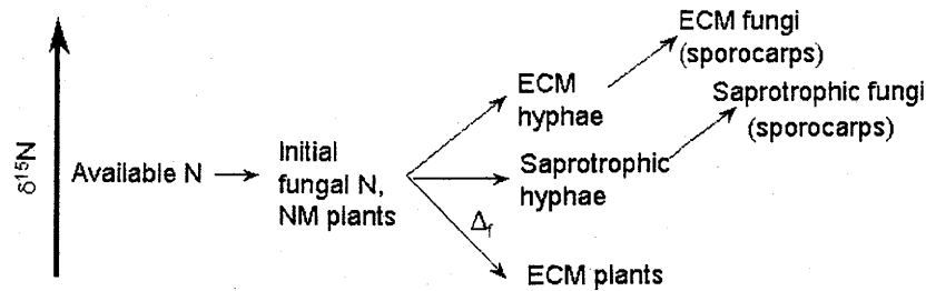
Fig. 4 Conceptual diagram of ^{15}\text{N} distribution patterns among available N, saprotrophic fungi, ectomycorrhizal (ECM) fungi, nonmycorrhizal plants (NM), and ectomycorrhizal plants. Fungi are separated into sporocarps and hyphae. ^{15}\text{N} enrichment occurs during sporocarp formation, ^{15}\text{N} depletion (designated \Delta_r ) occurs during creation of transfer compounds that are passed from mycorrhizal fungi to plants
