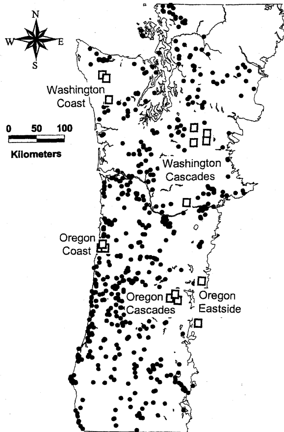
Fig. 1. Locations of Pacific Northwest old-growth forests for which total ecosystem C was determined (squares), and locations of pedons (dots) that were compared with STATSGO SOC (dots).
