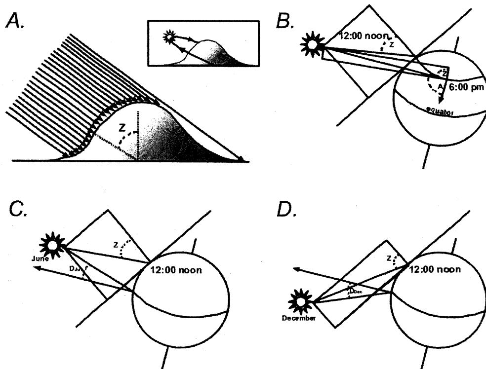
Figure 1.(A) Solar azimuth ( A ) and solar zenith angle ( Z ) create a topographic shading effect. (B) This shading is continuously shifting as the earth rotates causing changes in solar zenith and azimuth throughout the day. The change in the orientation of the earth's tilt in relation to the sun creates the basis for our seasons. The lower two panels depict the solar zenith ( Z ) and declination ( D ) for the same location during the summer (C.) and winter (D.) solstices.
