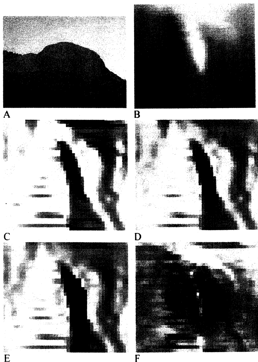
Figure 2.(A) Moro Rock is a large narrow granitic outcrop about 1.2 km long. The photo is from the west. The following maps are oriented towards the north. (B) DEM of the Moro Rock area is used to illustrate the differences between the radiation proxies draped over a drastic terrain feature (high elevations are lighter). (C) Transformed aspect map (high radiation areas are lighter). (D) Transformed aspect modified by slope. (E) Hillshade with A = 225 , S = 45 . (F) Potential relative radiation (PRR).
