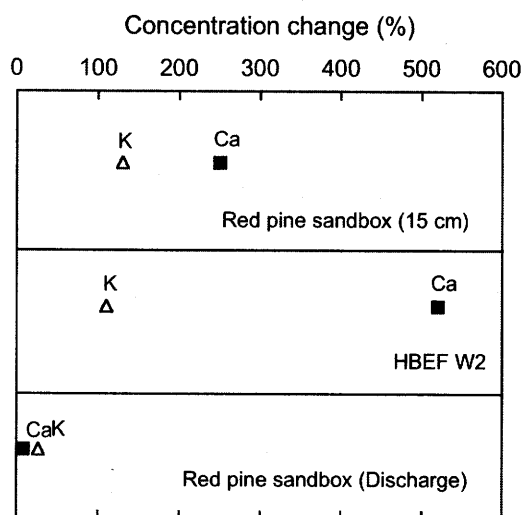
Figure 7. Comparison of change in nutrient concentrations after harvest experiments in Hubbard Brook Experimental Forest (HBEF) watershed 2 (W 2) and the RP sandbox. Change is defined as the difference between mean concentration values before and 32–36 months after harvest, divided by mean values before. K, potassium; Ca, calcium.
