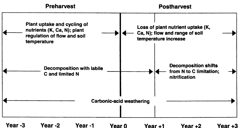
Figure 4. Conceptual model for progression of subsurface processes in response to aboveground biomass removal, based on results of the sandbox harvest experiment. K , potassium, Ca calcium, N nitrogen, C carbon.
