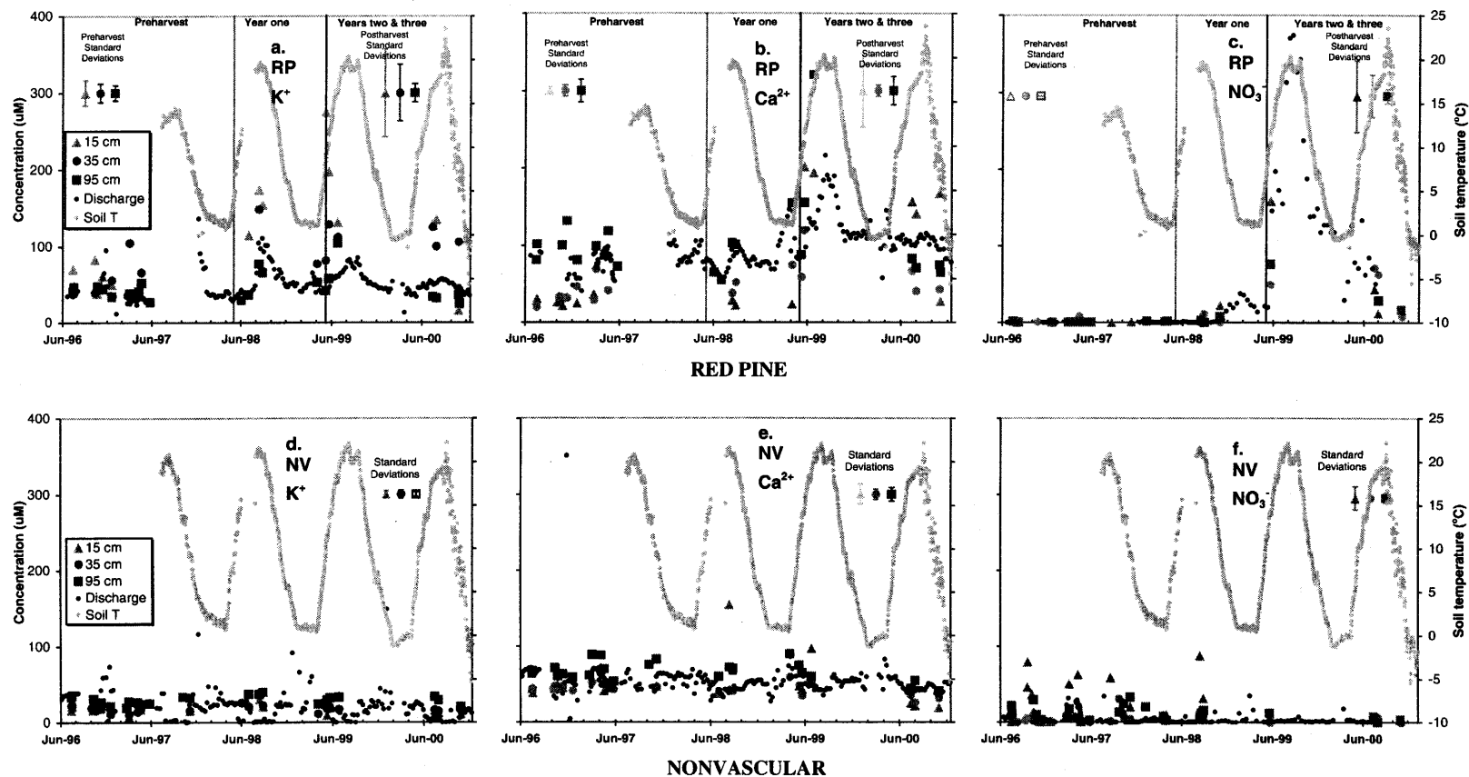
Figure 2. Nutrient concentrations over 5 years in RP and NV sandbox ecosystems. Red vertical line indicates harvest. Black dots represent sandbox discharge samples; color symbols represent soil-water samples at various depths (triangles: 15 cm; circles: 35 cm; squares: 95 cm). Standard deviations are reported among replicates. Soil temperature (grayscale) is at 95-cm depth. K, potassium, Ca, calcium, NO 3 , nitrate.
