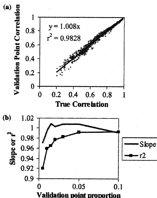
Figure 8. Summaries of tests of validation points for estimating true map correlation. (a) Plot of validation point vs. true correlation for validation point proportion of 0.03. Each point represents one map comparison. (b) Slope and r^2 of linear regressions of the type shown in (a), for a range of validation point proportions. Reasonable estimates of correlation are achieved with only 3–5% of plots used as validation points.
