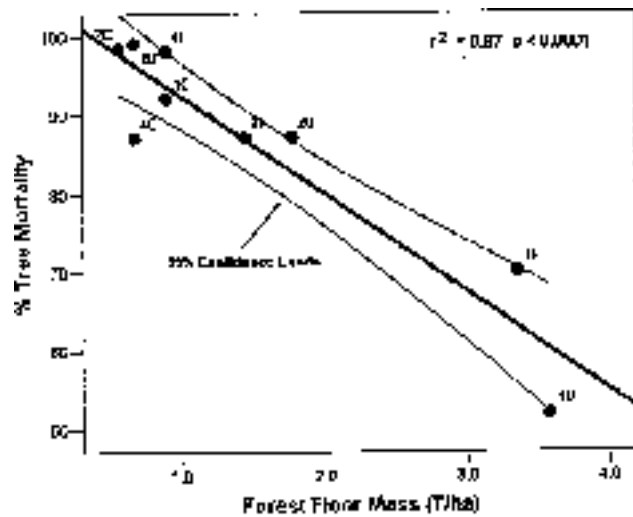
Figure 2. Correlation between forest floor mass one year post-fire (1997), and the percentage of dead trees in experimental units at Summit Fire study area, Malheur National Forest, northeastern Oregon.
