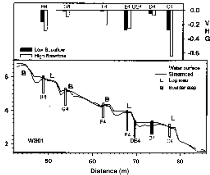
Figure 3. Longitudinal stream profile of WS1 in the region of the well network showing location of piezometers in the stream channel, the streambed surface and the stream water surface at low baseflow discharge (bottom panel) and the VHG through the streambed for each well at low- and high-baseflow discharge (top panel). Labels C4 through H4 designate streambed piezometers
