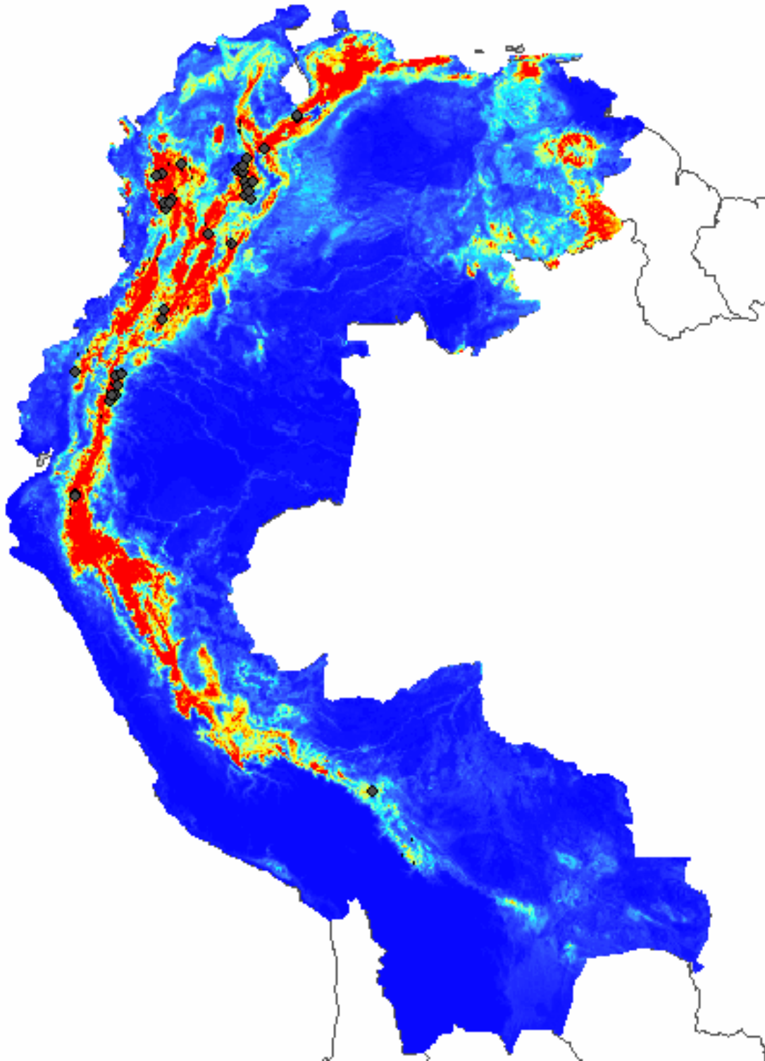
Figure 10. Intersection of Independent Cerulean Warbler Validation data set with output of MAXENT model. Dark circles indicate validation points where Cerulean Warblers were found.
