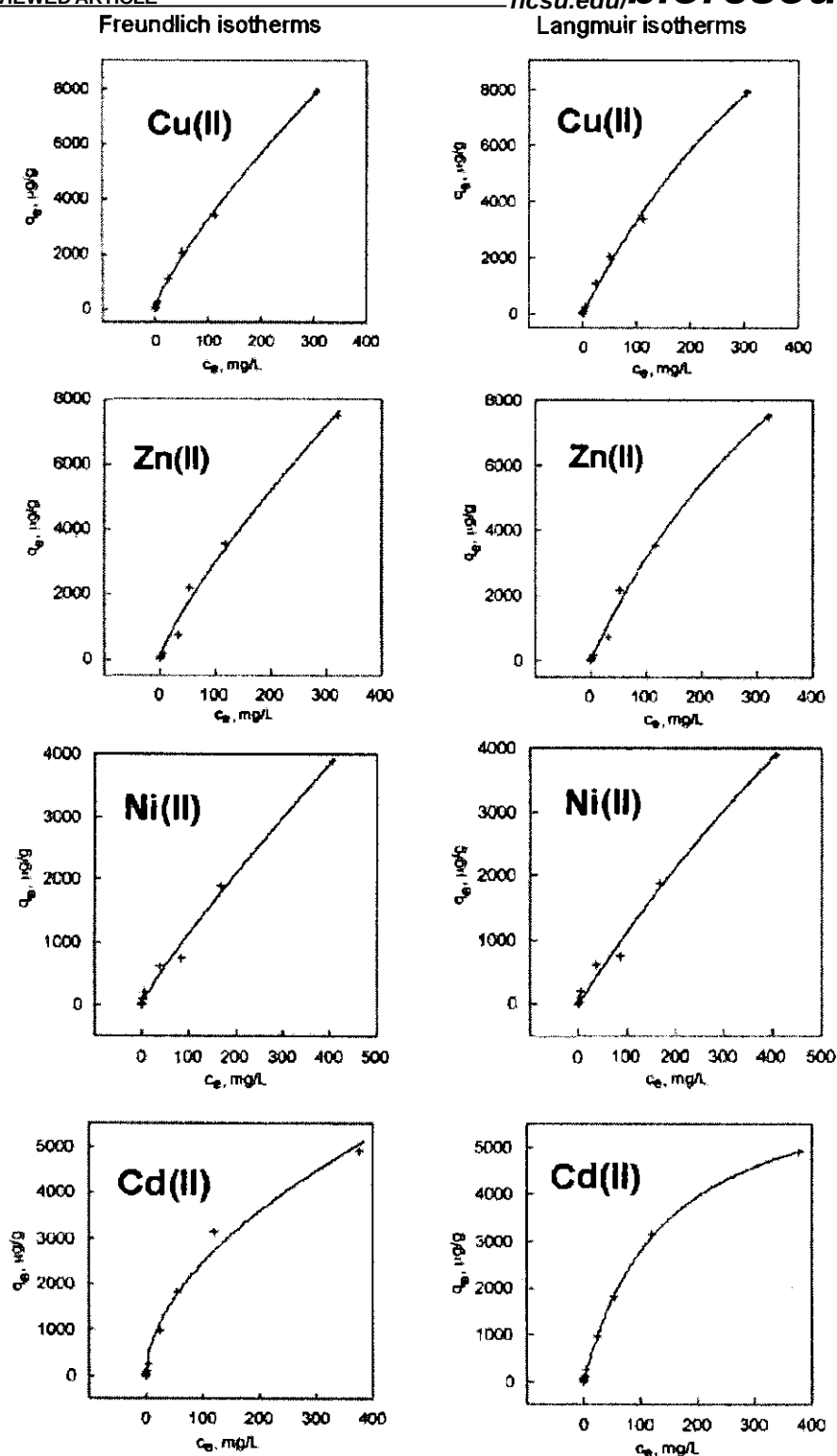
Fig. 2. Freundlich and Langmuir adsorption isotherms for Cu(II), Zn(II), Ni(II), and Cd(II) ions on pelletized bark. [Note: markers (+) represent experimental data points, and the lines (----) represent the fitted isotherms]
