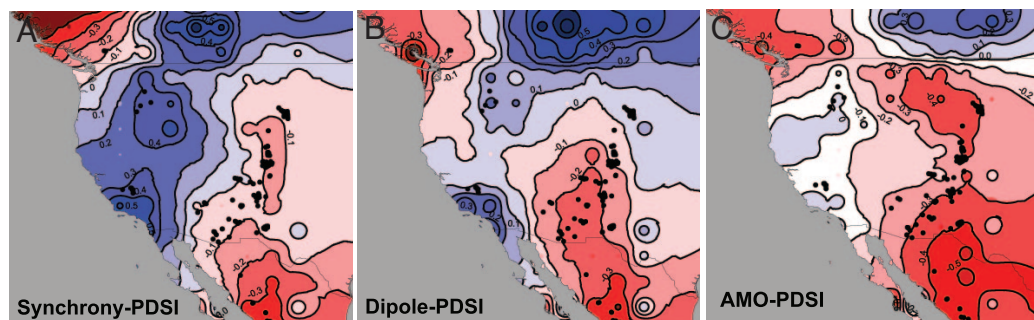
Fig. 4. Correlations between the fire synchrony index (A), the dipole fire index (B), and the 49-year running mean AMO (C) with a time-smoothed version (49-running mean) of gridded tree-ring reconstructed PDSI for the period 1574–1899.
