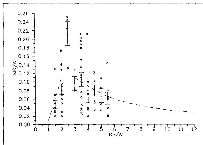
Figure 3— The ratio of migration rate ( MR ) to channel width ( W ) plotted against the ratio of radius of curvature ( R_c ) to width. The asterisks and bars represent the means and standard errors, respectively. The curves are from Nanson and Hickin (1986).
