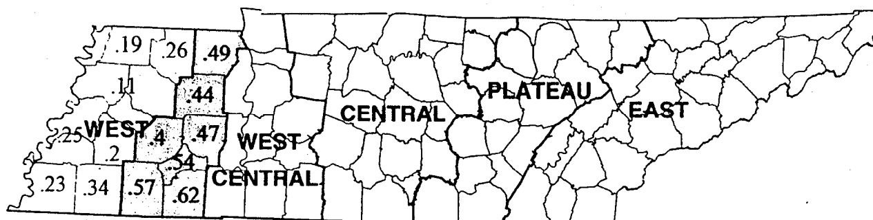
Figure 1.—Example of how to group counties in survey unit 1, Tennessee for development of correction factors based on one panel of data. Shaded counties are aggregated for a common correction factor.
