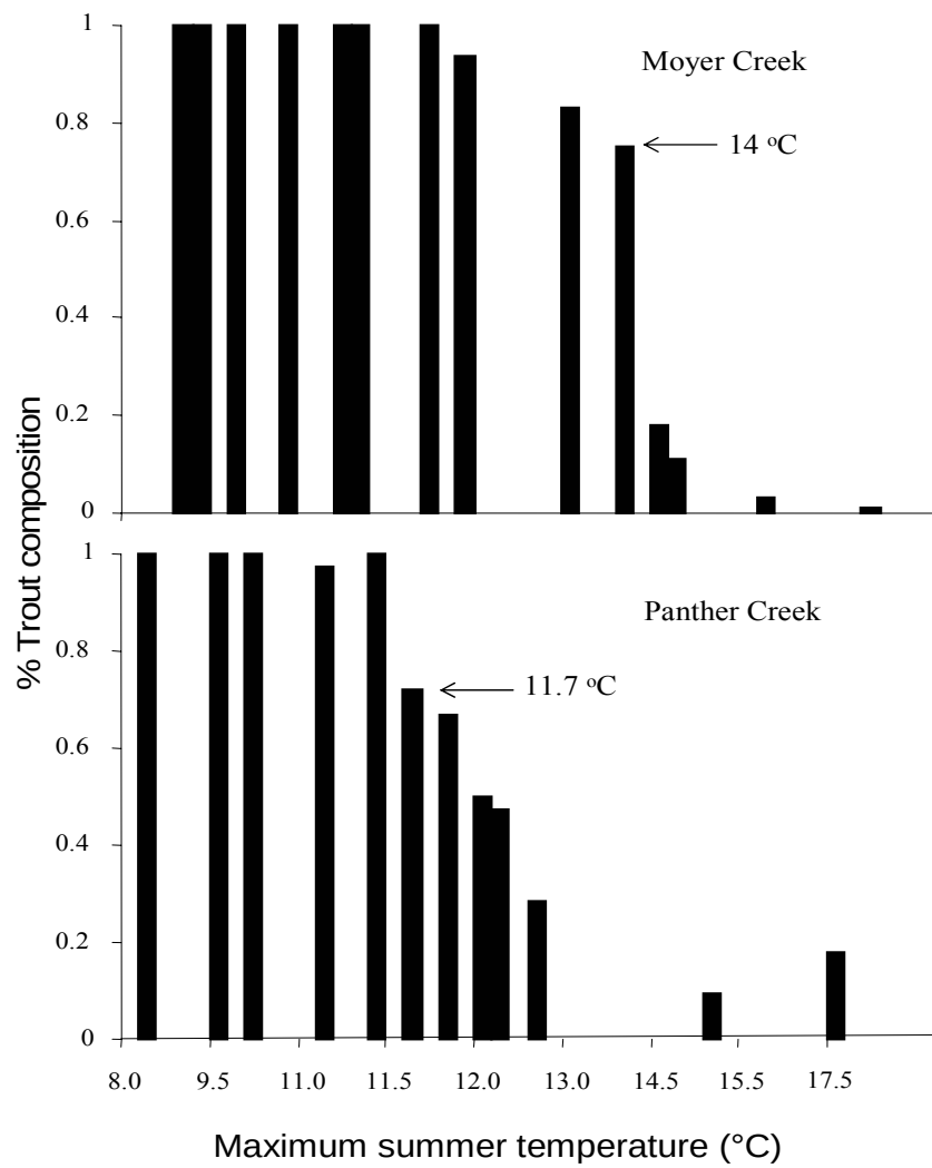
Figure 6. Thermal shift in numerical dominance of bull trout in the presence of brook trout (Panther Creek) compared to a stream where no brook trout were found (Moyer Creek).
