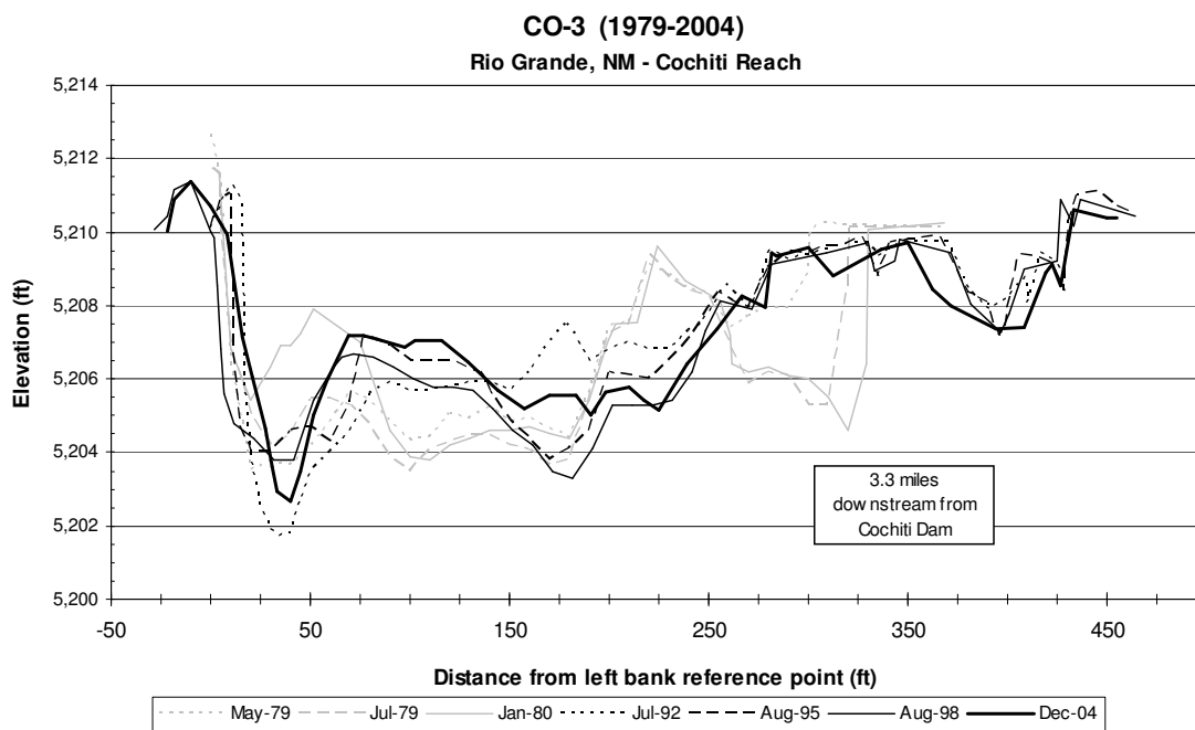
Figure B-6 Post-dam conditions (April 1979 to December 2004)
