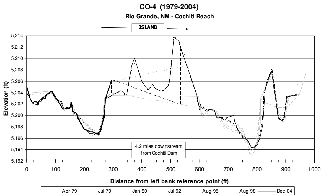
Figure B-9 Post-dam conditions (April 1979 to December 2004)
