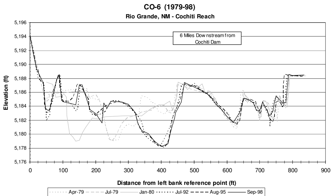
Figure B-15 Post-dam conditions (April 1979 to September 1998)
