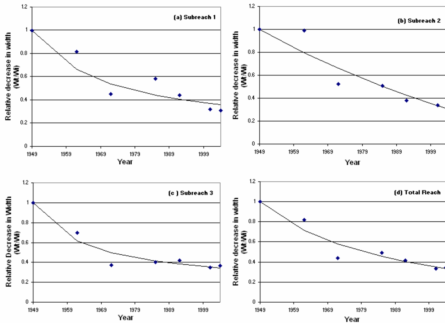
Figure 4-10 Hyperbolic fits to relative decreases in width from 1949 to 2004 for (a) subreach 1, (b) subreach 2, (c) subreach 3, and (d) the entire Cochiti Dam reach.
