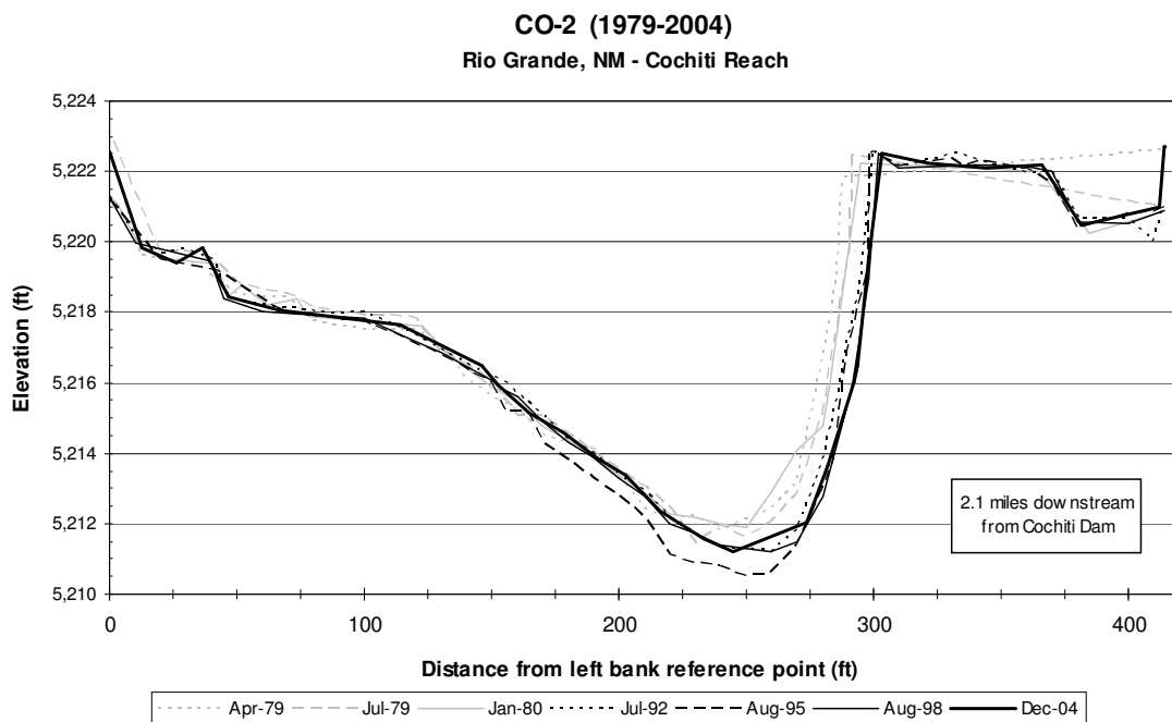
Figure B-3 Post-dam conditions (April 1979 to December 2004)
