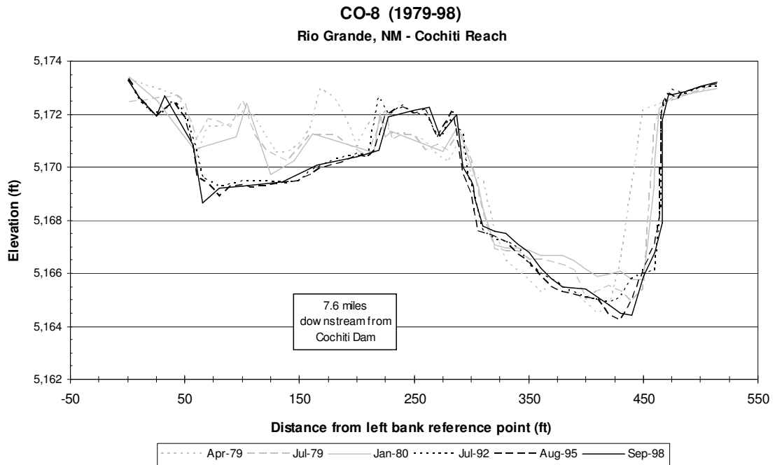
Figure B-21 Post-dam conditions (April 1979 to September 1998)
