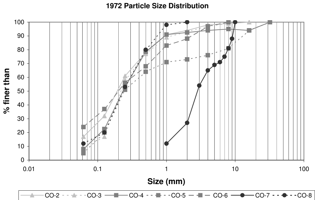
Figure D-1 Particle Size Distribution in the Cochiti Dam reach for 1972. Triangles denote subreach 1, squares denote subreach 2, and circles denote subreach 3.
