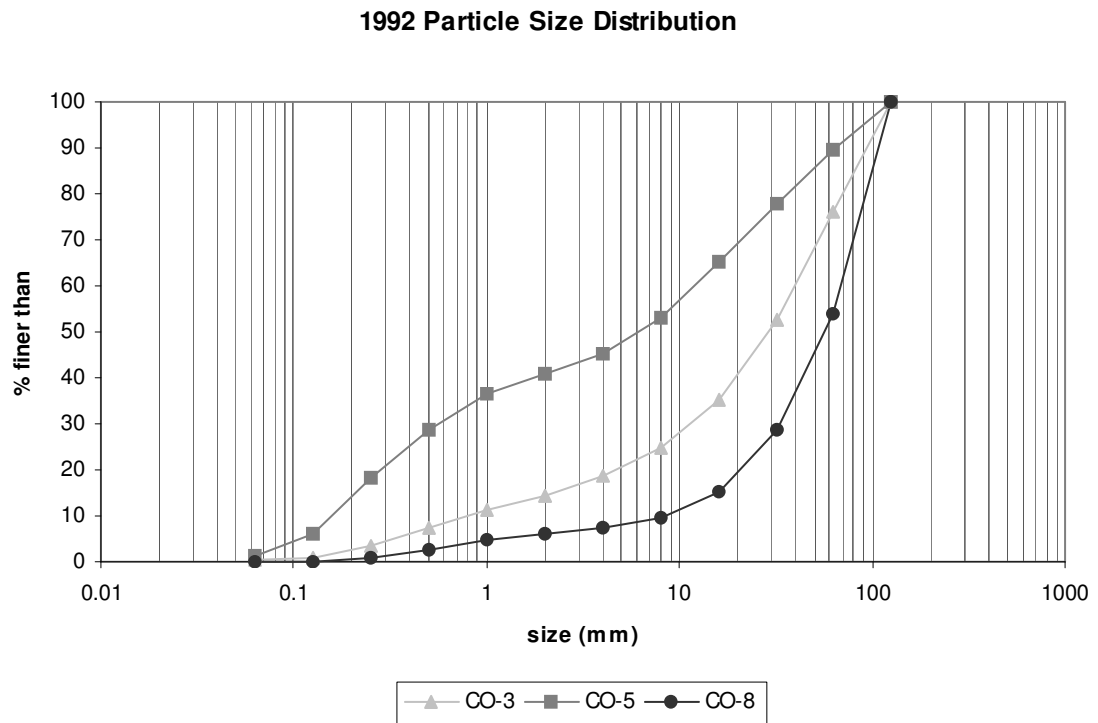
Figure D-2 Particle Size Distribution in the Cochiti Dam reach for 1992. Triangles denote subreach 1, squares denote subreach 2, and circles denote subreach 3.
