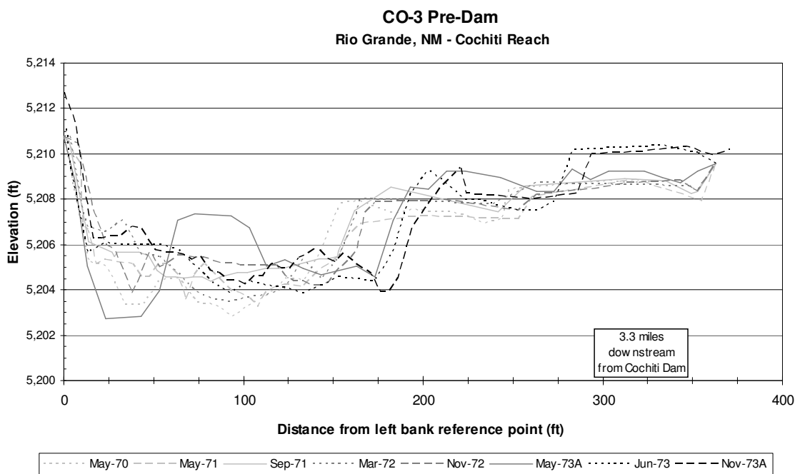
Figure B-4 Pre-dam conditions (all cross-sections up to Nov. 1973)
