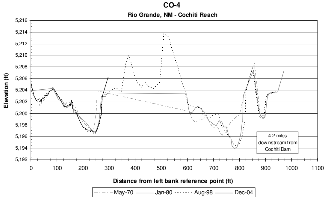
Figure 3-12 Thalweg change at CO-4
