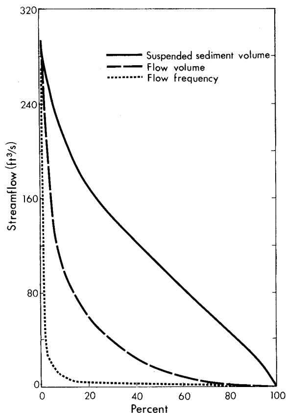
Figure 2 —Flow and sediment regimes of South Fork Caspar Creek showing the percentage of the flow frequency, flow volume, and sediment volume occurring at higher discharges than the level indicated. For example: about 80 percent of the sediment transport takes place in flows greater than 40 ft³/s.
