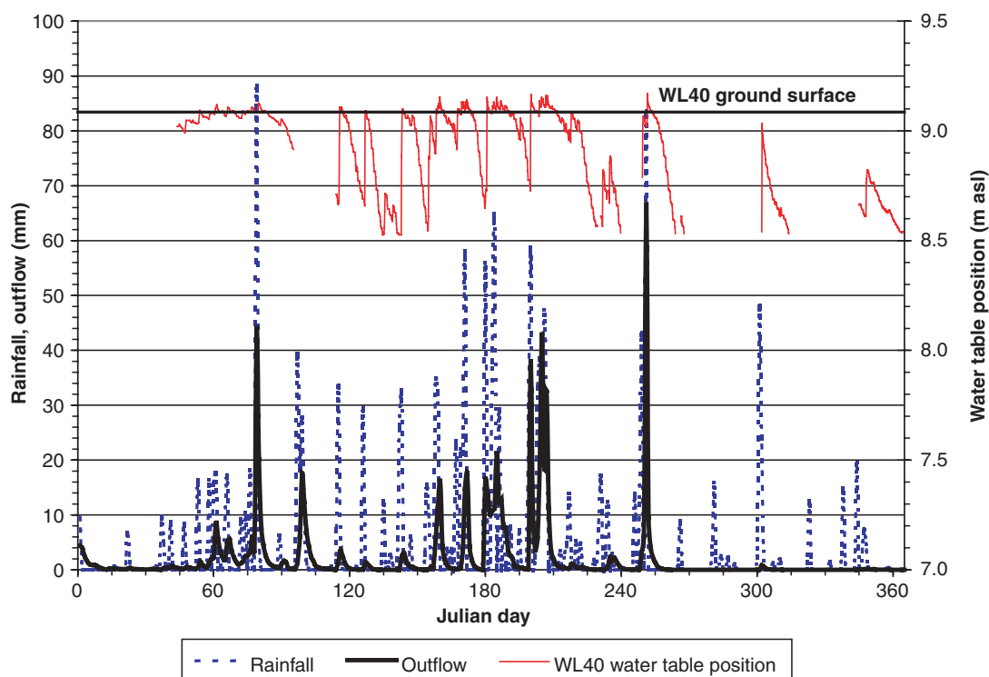
FIGURE 3. 2003 Daily Rainfalls, Outflows, and Water Table Position.
