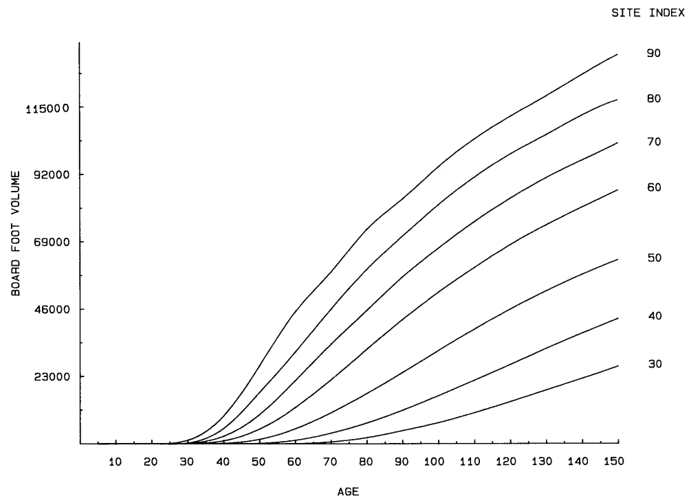
Figure 31—Grand fir yield curves for unthinned plantations in Inland Northwest forests (merchantable board feet [Scribner] 4.5-inch top, stems greater than 7 inches d.b.h.).
