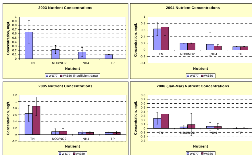
Figure 2. Comparison of annual average nutrient concentrations between WS 77 and WS 80. Data for WS 80 in 2003 was not available.
