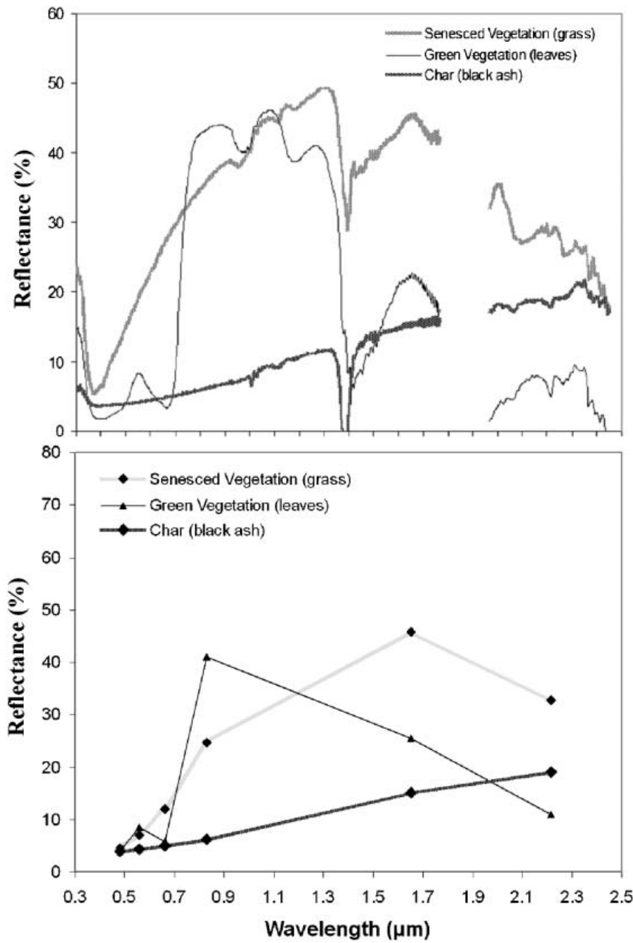
Figure 2. Generic spectral reflectance curves of green vegetation, senesced vegetation, and char (black ash). Spectra were acquired by Smith et al. (2005) from a woodland savannah environment. The data gap at \sim 1.8\mu\text{m} represents the dominant atmospheric water absorption feature where data quality is insufficient for analysis. Lower figure shows the Landsat band equivalent spectra applied in the unmixing.
