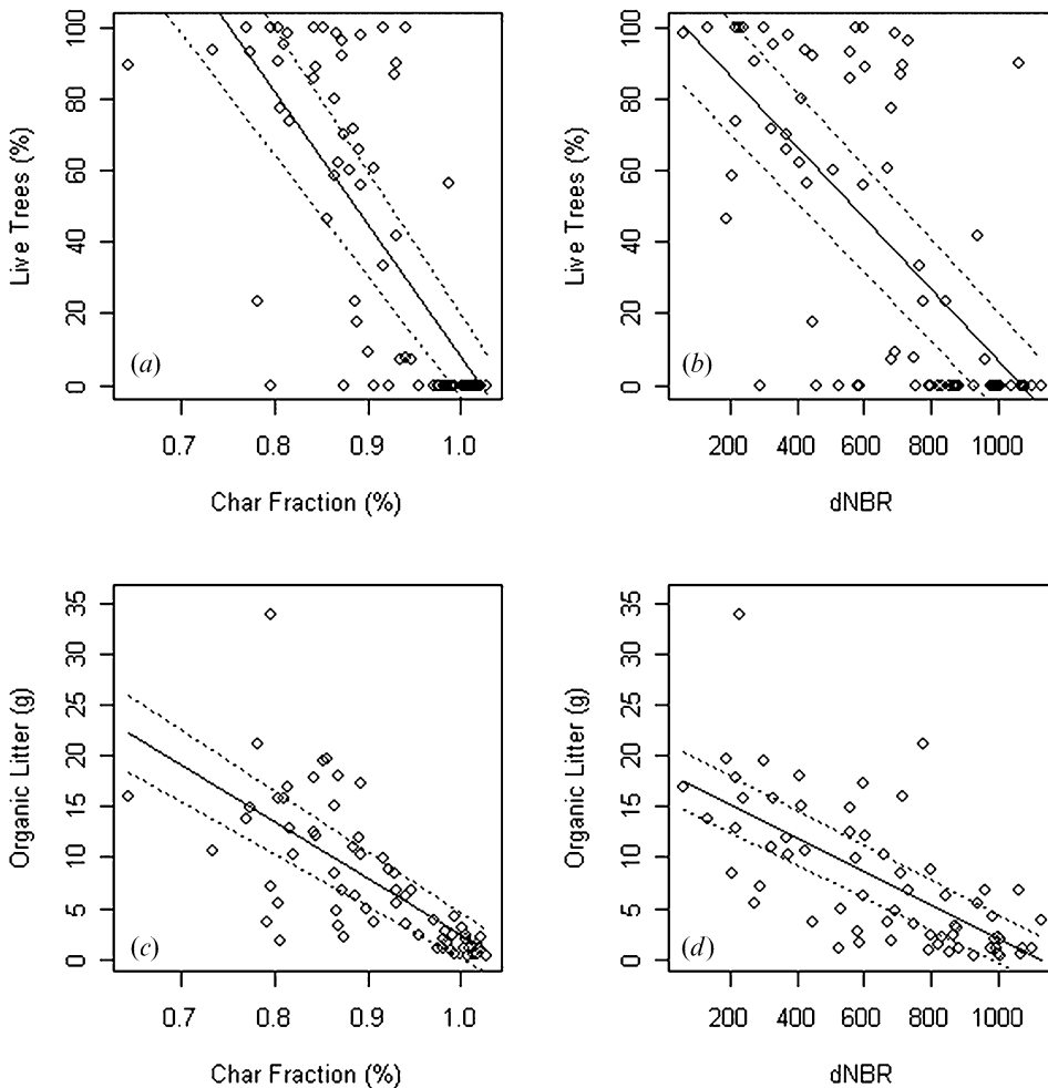
Figure 3. Scatter plots depicting the relationships between each immediate (Year 0) remote post-fire measure and canopy and sub-canopy one-year post-fire indicators of ecosystem conditions. In each case the solid line represents the linear line-of-best-fit. Regression statistics: (A) r^2=0.56 , \text{SE}=28.03 , y=-370 \cdot x+378 ; (B) r^2=0.55 , \text{SE}=29.69 , y=-0.10 \cdot x+103.9 ; (C) r^2=0.55 , \text{SE}=4.78 , y=-58 \cdot x+61 ; and (D) r^2=0.52 , \text{SE}=8.01 , y=-0.02 \cdot x+24.1 . The dashed lines indicate in each case the 95% confidence intervals.
