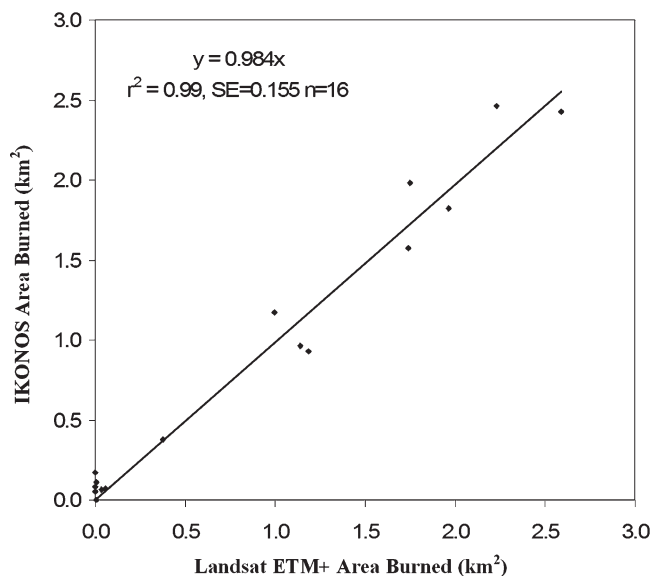
Figure 4. Regression of IKONOS and Landsat area burned for 16 regular grid squares derived from figure 3(b) and (d). Line of best fit is depicted and regression was significant at the 95% confidence level.
