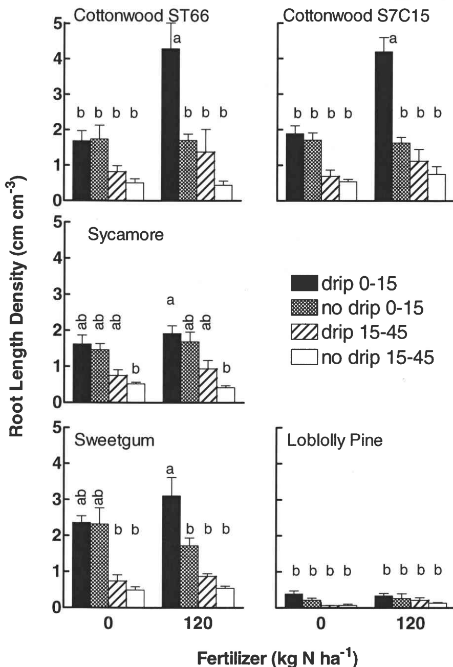
Fig. 6 Fine-root density distribution in 2003 for five tree genotypes. Sample locations 4 and 5 (see Fig. 1) under the drip tube (drip) were compared to sample locations 2 and 3 between drip tubes (no drip). The surface mineral soil layer (0–15 cm) was compared to the subsurface soil layer (15–45 cm). Each bar is the mean \pm standard error of three replicate plots for irrigation treatments ( n=6 ). Bars topped by the same letter for each genotype are not significantly different (Tukey's HSD, \alpha=0.05 )
